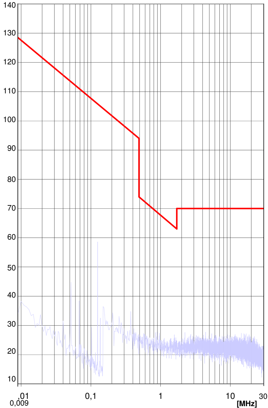
Picture: 5-1 Radiated field strength 0,009 MHz – 30 MHz (pre scan)
