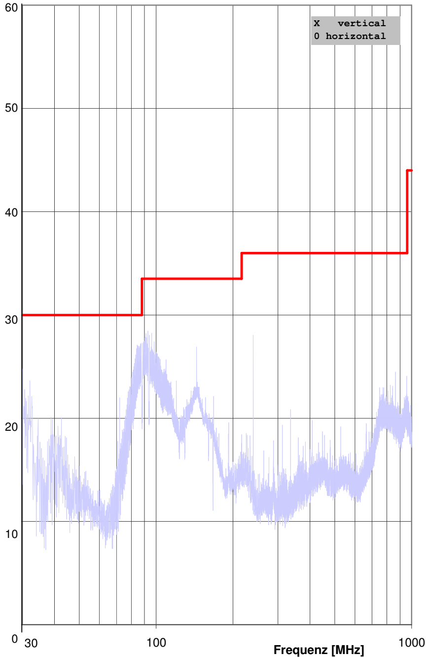
Picture: 5-3 Radiated emission 30 MHz – 1000MHz (pre scan)
