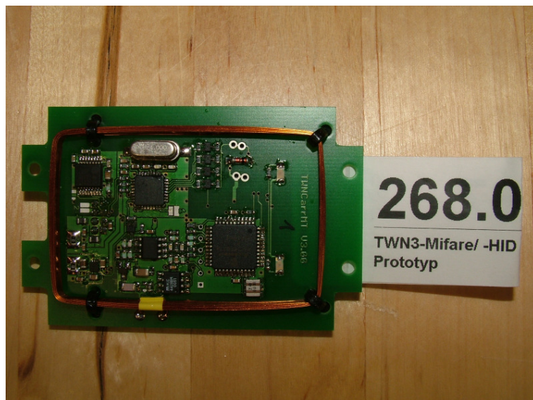
Picture 1: EUT TWN3 Reader Multitag (TWN3MT)
