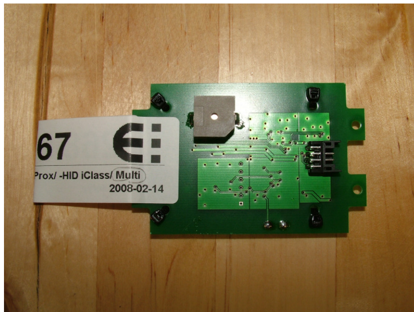
Picture 1-1: TWN3 Reader Multitag (TWN3MT) top side
