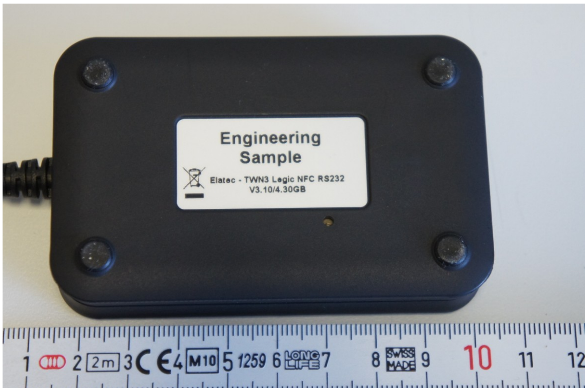
Picture 6: EUT with serial connector (rear)
