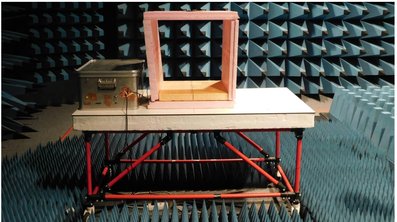
Picture 5: AC, radiated emission test 1 GHz – 25 GHz (front view)
