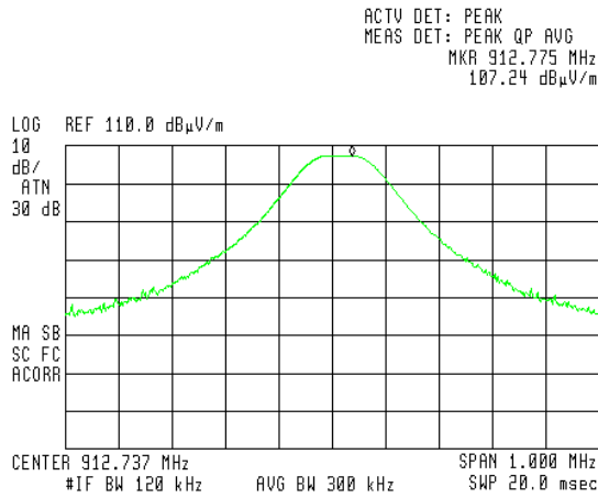
Figure 27 — 912.75 MHz-Horizontal
