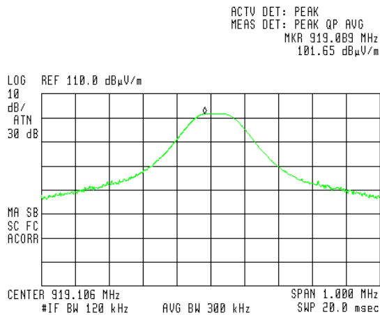
Figure 29 — 919.106 MHz VERTICAL
