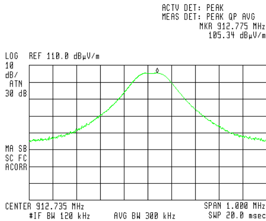
Figure 28 — 912.75 MHz-Vertical
