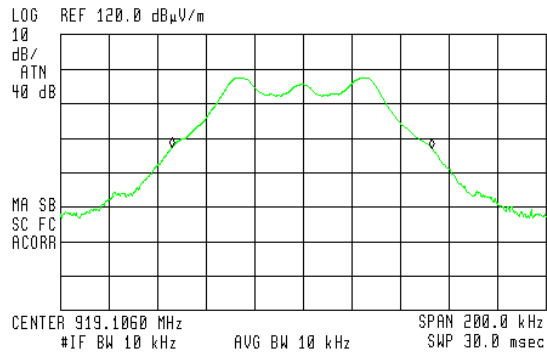
Figure 8. — 919.106 MHz
