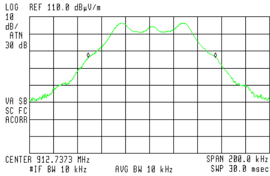
Figure 7. — 912.75 MHz
