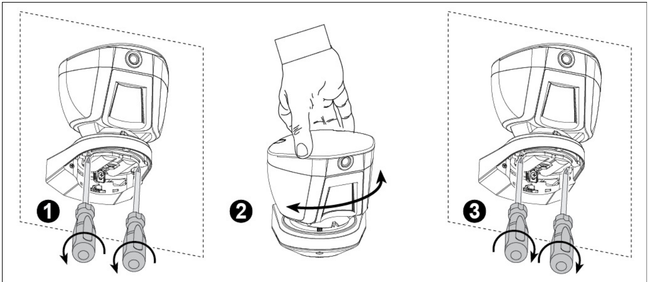
Figure 2 - Installation
