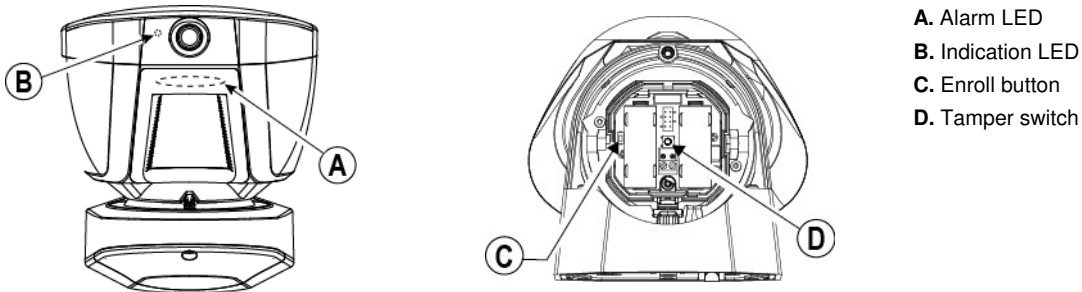
Figure 5. TOWER CAM PG2
