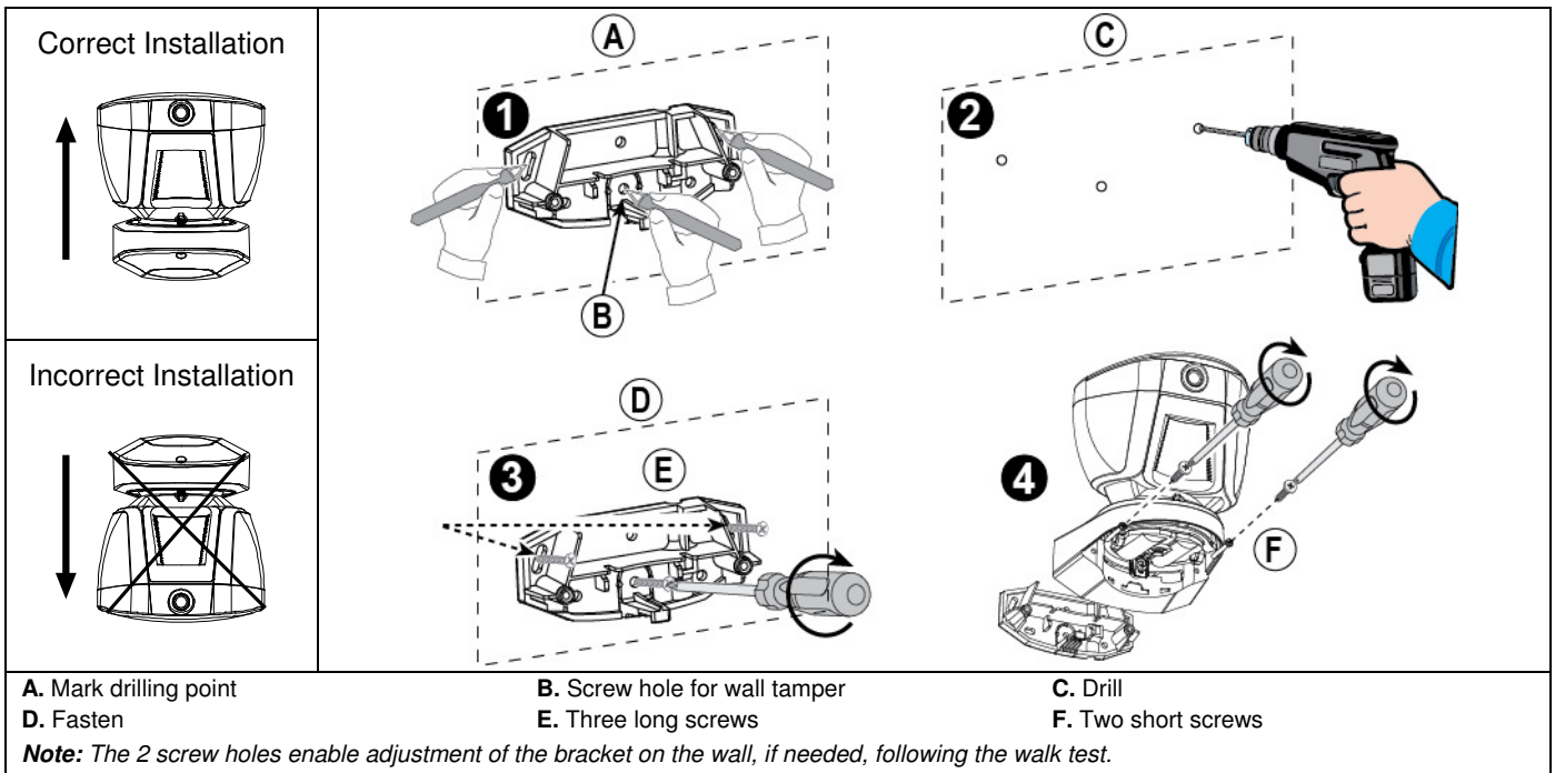
Figure 2 - Installation
