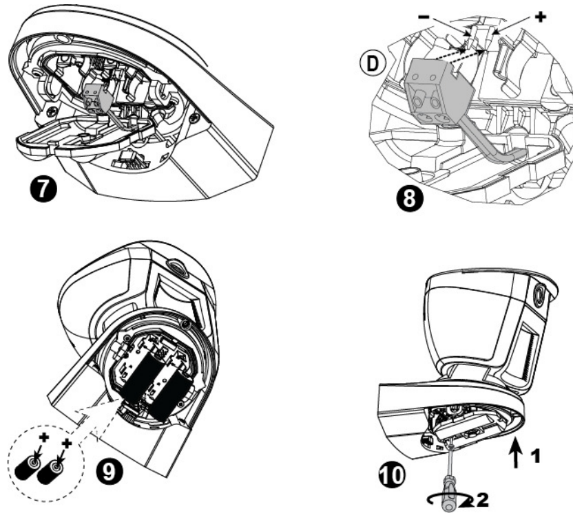
Figure 4 – Battery Insertion
