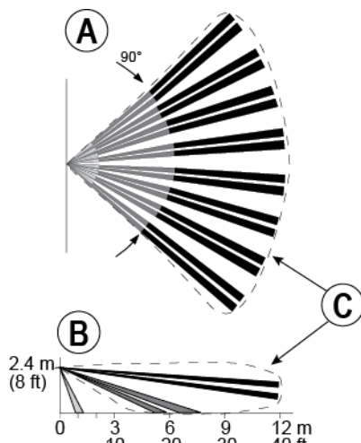
Figure 6. Coverage Pattern
