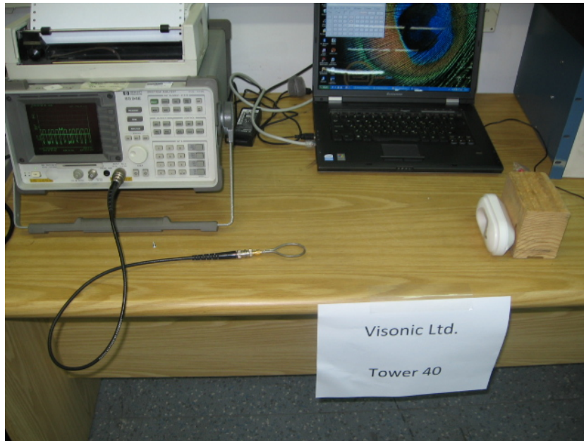
Figure 1. Radiated Emission Tests
