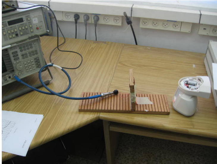
Figure 1. Table Top Radiated Emission Test
