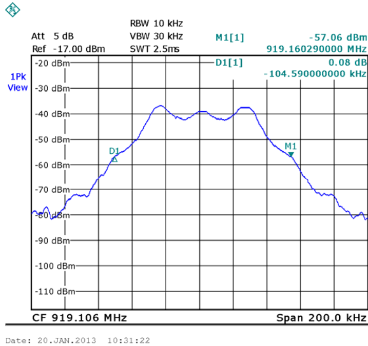
Figure 7. — 919.106 MHz
