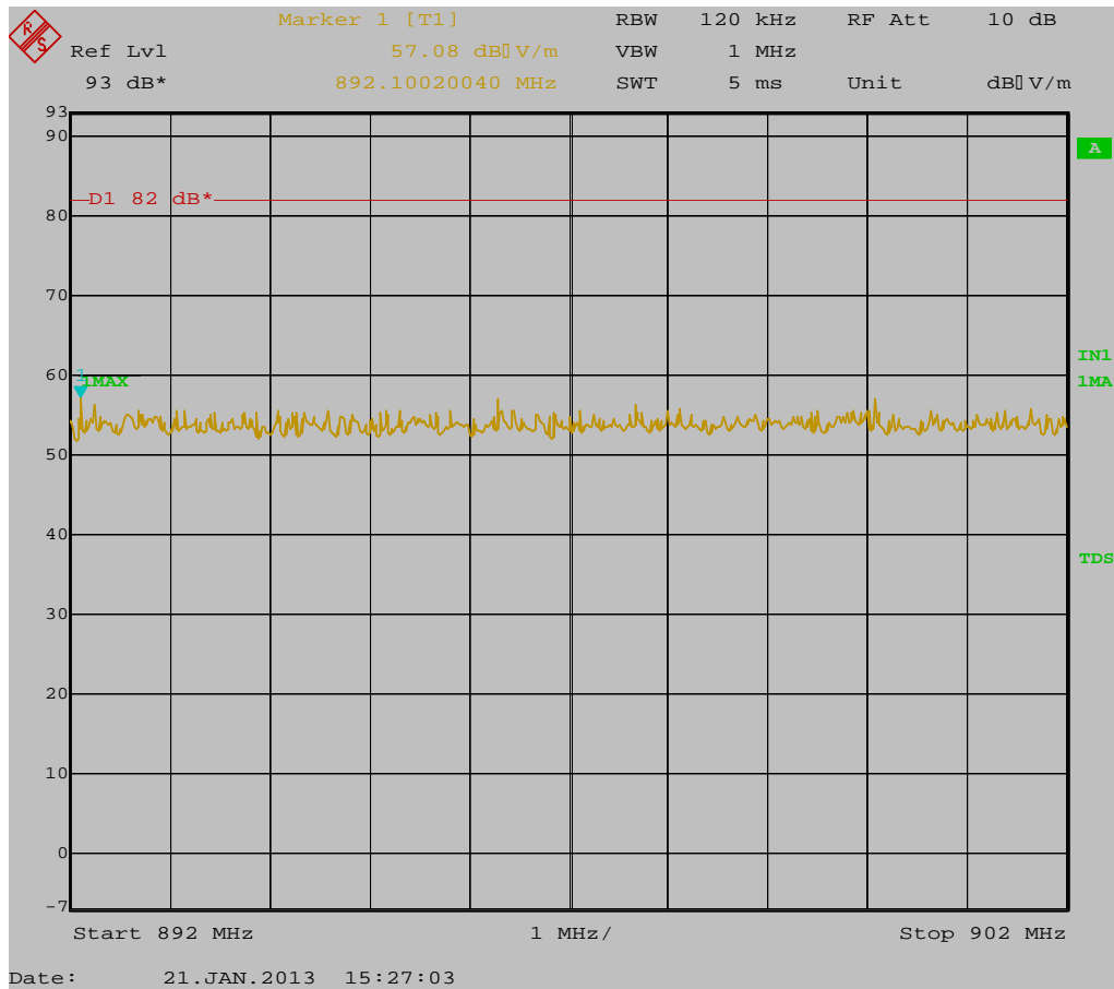
Figure 30 — 912.75 MHz
