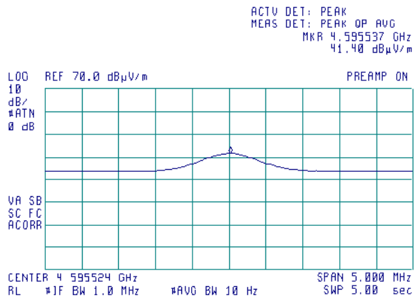
Plot 7.7.26 Radiated emission measurements at the sixth harmonic of low carrier frequency
