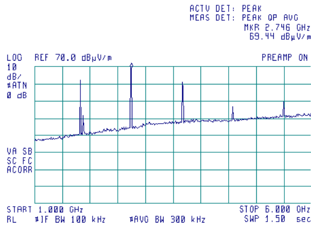
Plot 7.7.10 Radiated emission measurements from 1000 to 6000 MHz at the high carrier frequency
