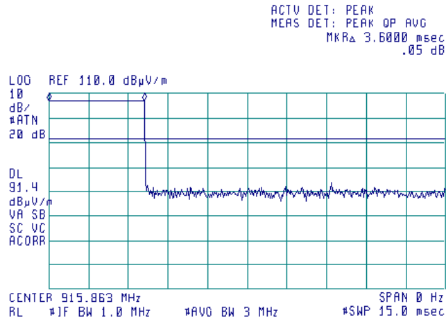
Plot 7.7.42 Transmission pulse period
