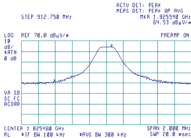
Plot 7.7.15 Radiated emission measurements at the second harmonic of mid carrier frequency
