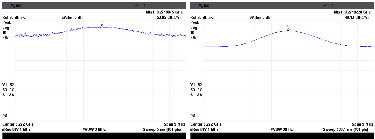
Plot 7.7.38 Radiated emission measurements at the tenth harmonic of low carrier frequency
