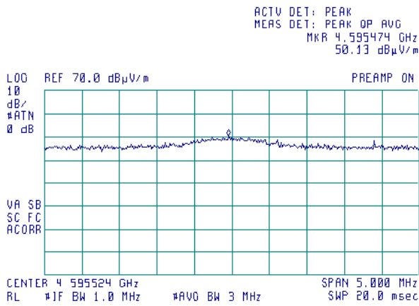
Plot 7.7.26 Radiated emission measurements at the sixth harmonic of low carrier frequency
