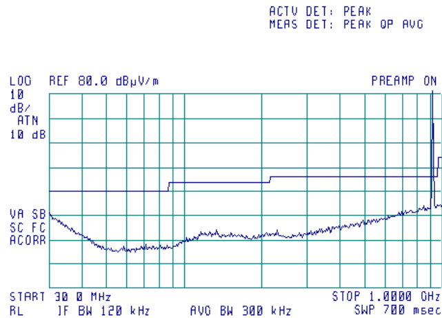
Plot 7.7.7 Radiated emission measurements from 30 to 1000 MHz at the mid carrier frequency
