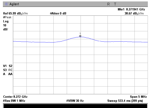
Plot 7.7.34 Radiated emission measurements at the tenth harmonic of low carrier frequency
