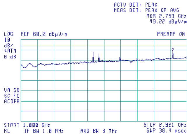
Plot 7.7.11 Radiated emission measurements from 1000 to 2900 MHz at the high carrier frequency
