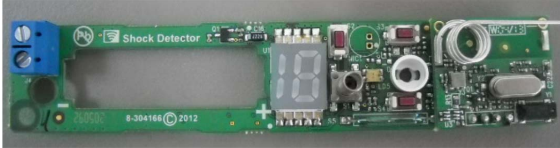
Photograph No.2 Shock detector SD-304C PG2 main PCB with RF card front view
