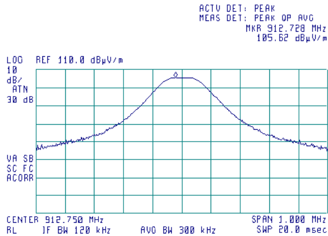
Plot 7.5.2 Field strength of carrier at mid frequency and Unom
