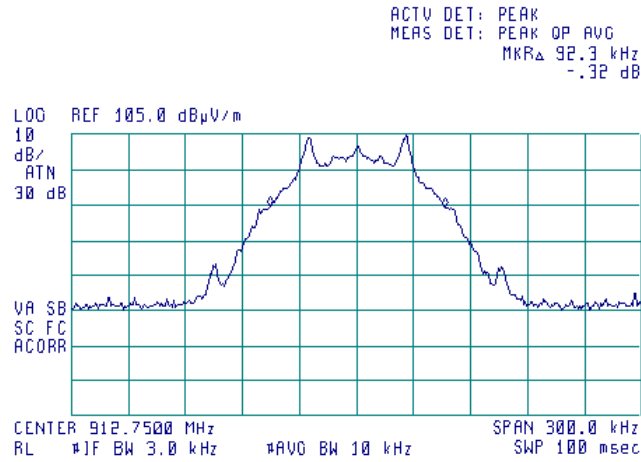
Plot 7.1.2 20 dB bandwidth test result at mid frequency
