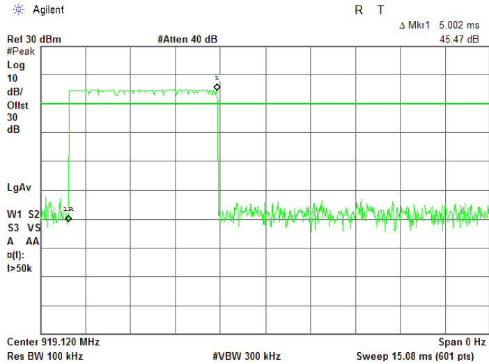
Plot 7.8.31 Transmission pulse duration
