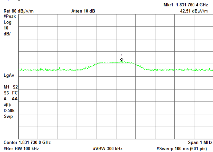
Plot 7.8.16 Radiated emission measurements at the third harmonic of low carrier frequency
