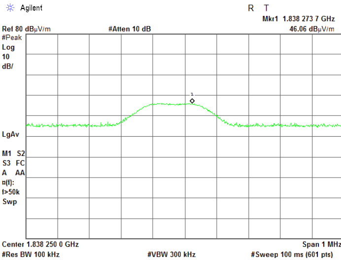
Plot 7.8.18 Radiated emission measurements at the third harmonic of mid carrier frequency
