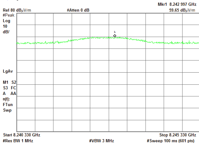
Plot 7.8.28 Radiated emission measurements at the ninths harmonic of high carrier frequency
