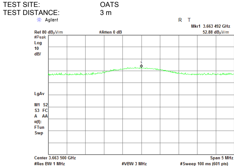
Plot 7.8.19 Radiated emission measurements at the fourth harmonic of mid carrier frequency
