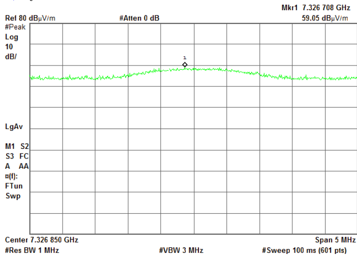
Plot 7.8.26 Radiated emission measurements at the ninths harmonic of low carrier frequency
