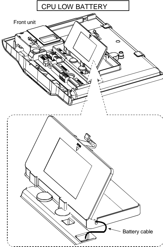
Figure 10. Battery Replacement
