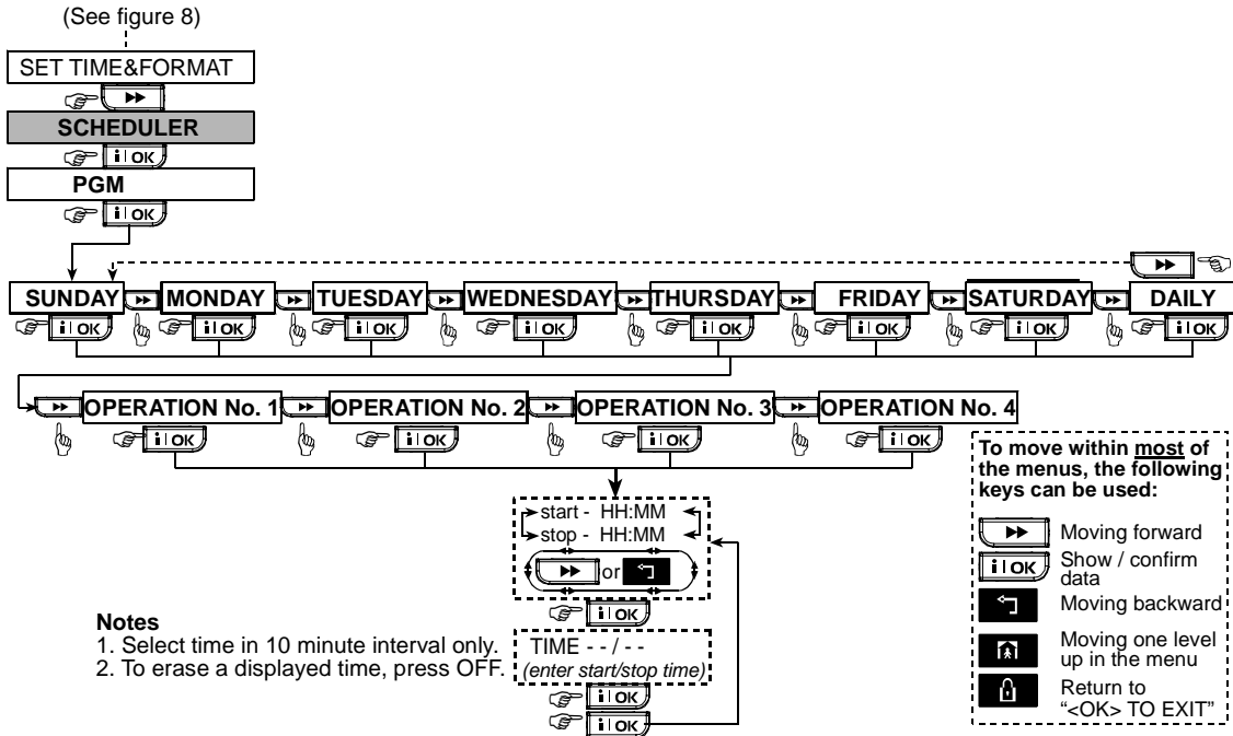
Figure 8 DETAIL "A" - Scheduler Function
