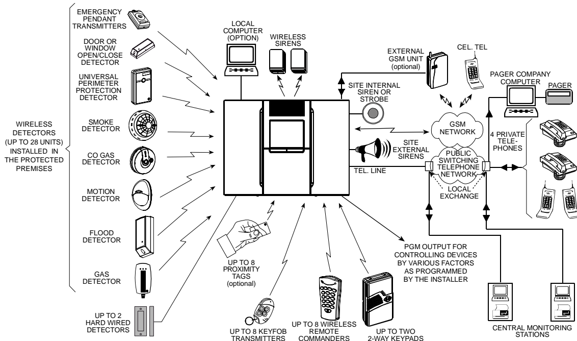
Figure 2. System Configuration
