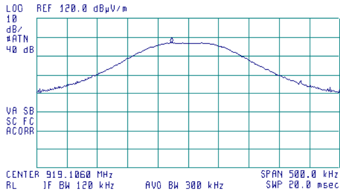
Plot 7.5.12 Field strength of carrier at high frequency at horizontal antenna polarization
