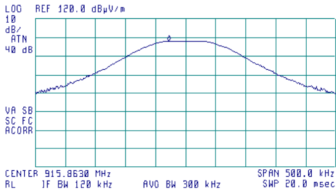
Plot 7.5.8 Field strength of carrier at mid frequency at horizontal antenna polarization
