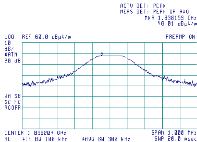
Plot 7.6.18 Radiated emission measurements at the third harmonic of low carrier frequency
