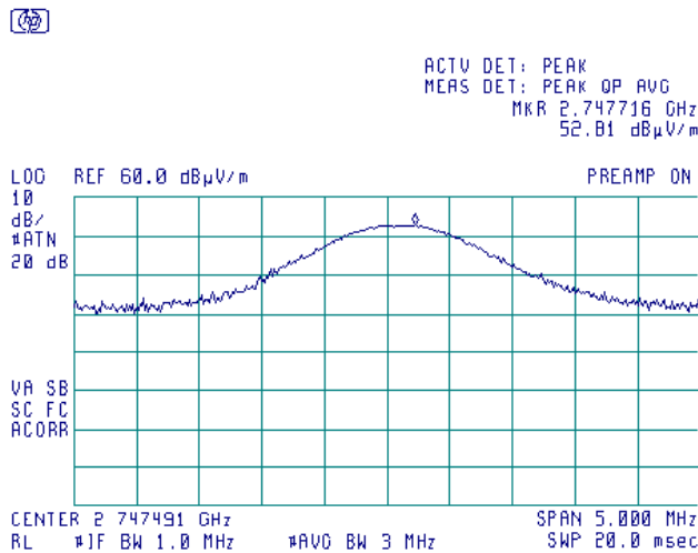
Plot 7.6.20 Radiated emission measurements at the third harmonic of high carrier frequency
