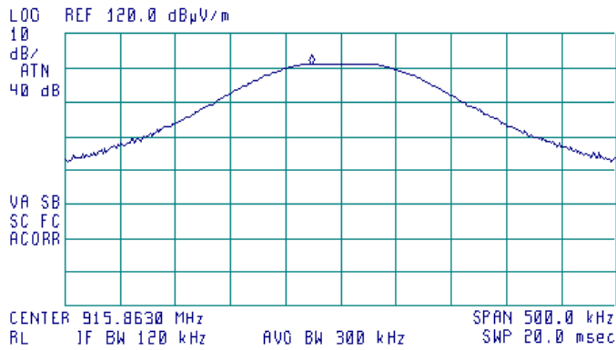
Plot 7.5.6 Field strength of carrier at mid frequency at horizontal antenna polarization
