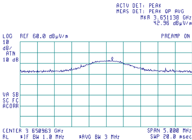
Plot 7.6.22 Radiated emission measurements at the fourth harmonic of mid carrier frequency
