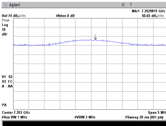
Plot 7.6.36 Radiated emission measurements at the ninth harmonic of low carrier frequency
