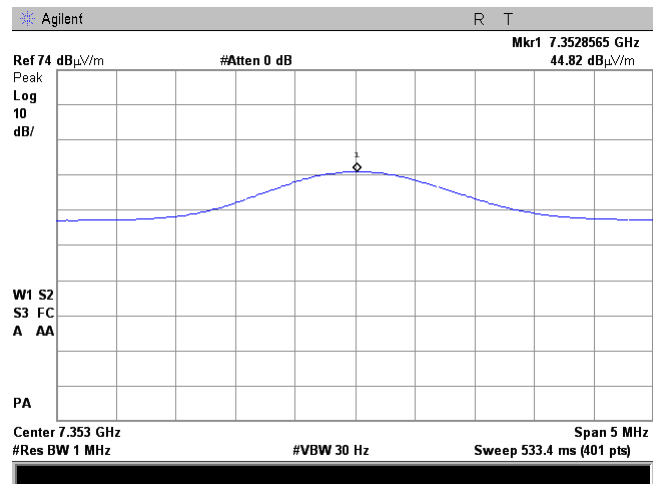
Plot 7.6.36 Radiated emission measurements at the ninth harmonic of low carrier frequency
