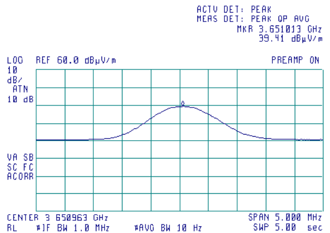
Plot 7.6.22 Radiated emission measurements at the fourth harmonic of mid carrier frequency
