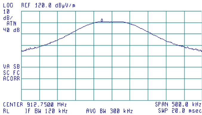
Plot 7.5.2 Field strength of carrier at low frequency at horizontal antenna polarization
