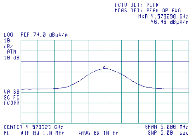
Plot 7.6.26 Radiated emission measurements at the fifth harmonic of high carrier frequency
