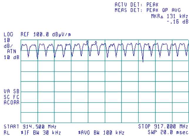
Plot 7.3.2 Number of hopping frequencies in the frequency range 914.5 –917.0 MHz (nineteen)
