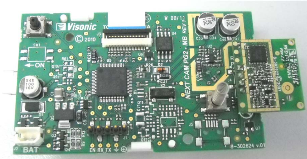
Photograph No.5 Detector main PCB second side view
