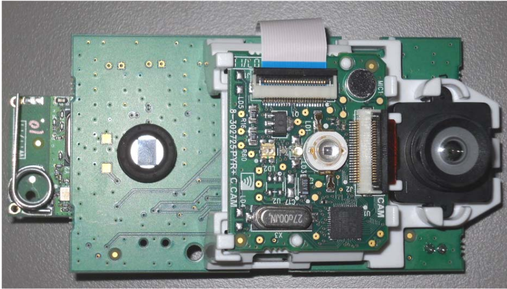
Photograph No.3 Digital PIR detector with camera PCBs front view
