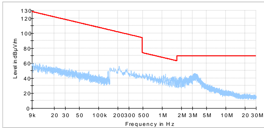
Low, mid, high carrier frequency
