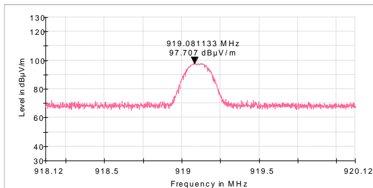
Plot 7.5.3 Field strength of carrier at high frequency
