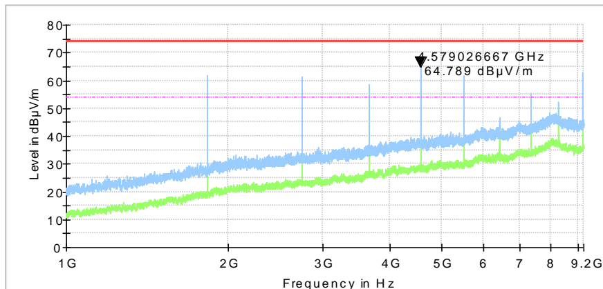
Mid carrier frequency
