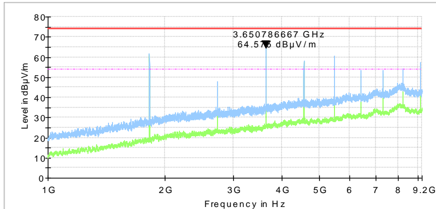
Low carrier frequency
