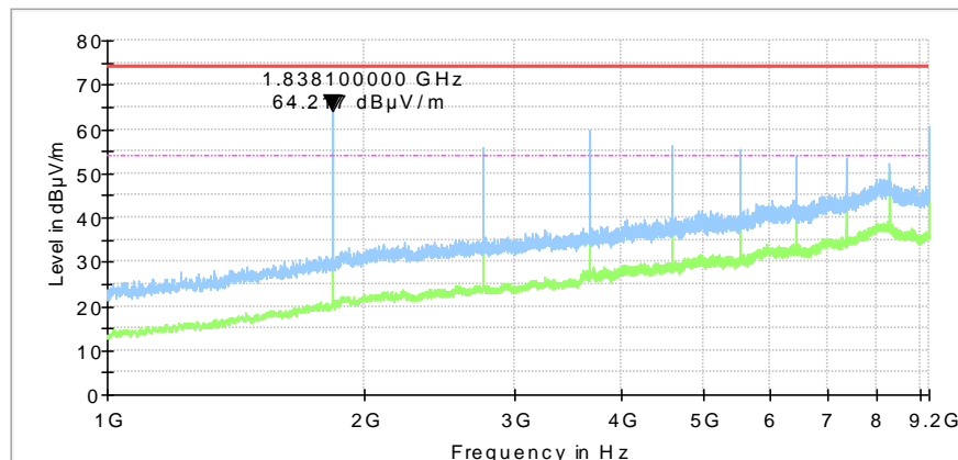
High carrier frequency
