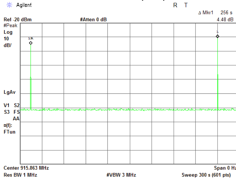
Plot 7.6.5 Transmission pulse period
