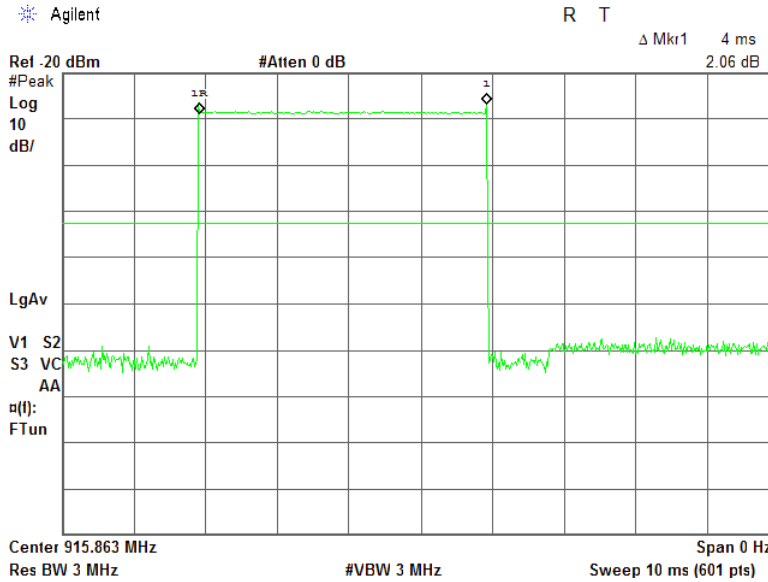
Plot 7.6.4 Transmission pulse duration
