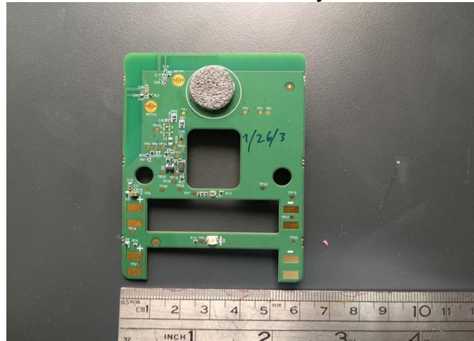
Photograph No.4 Antenna assembly
