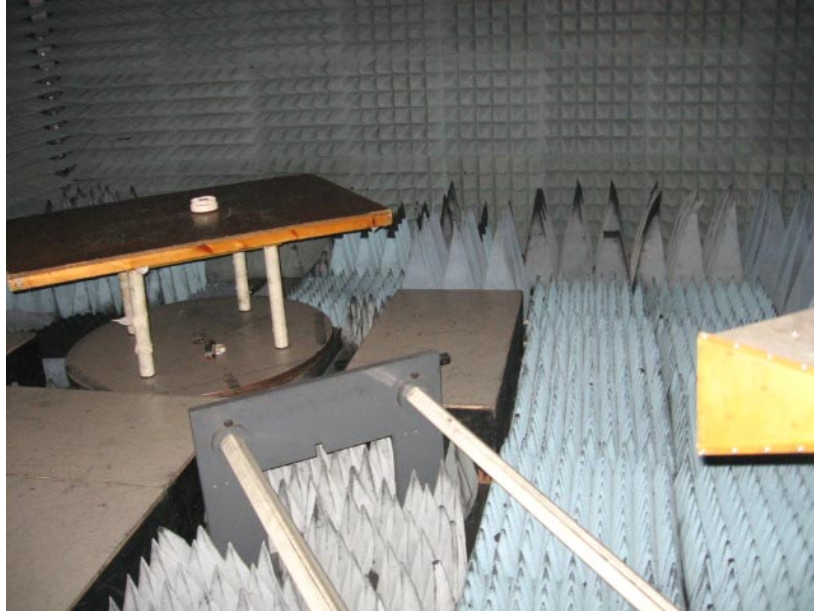
Photograph No.3 Setup for carrier and spurious emission field strength measurements in the anechoic chamber above 1000 MHz range
