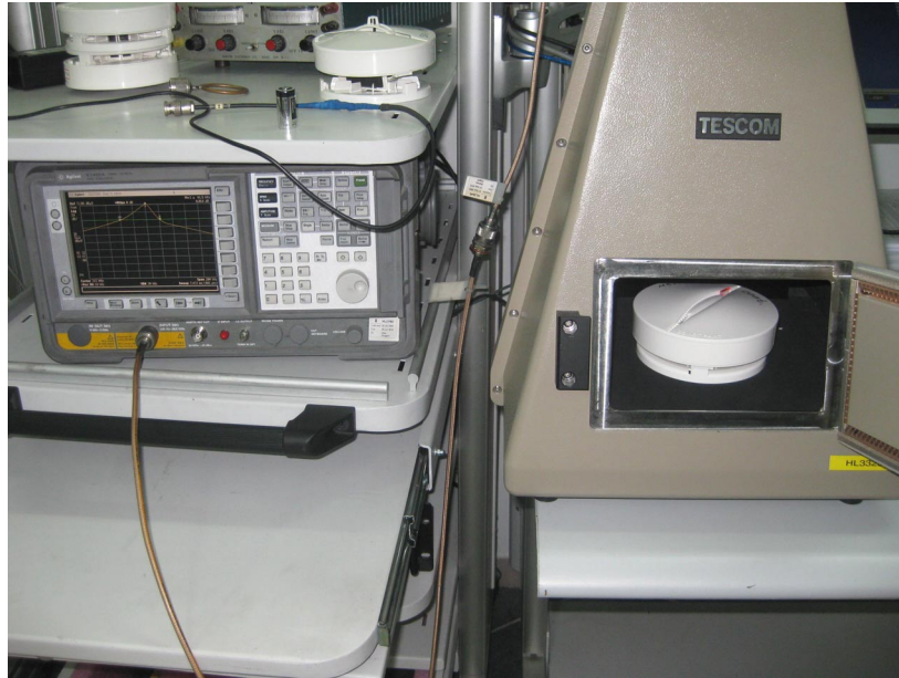
Photograph No.5 Setup for occupied bandwidth measurements
