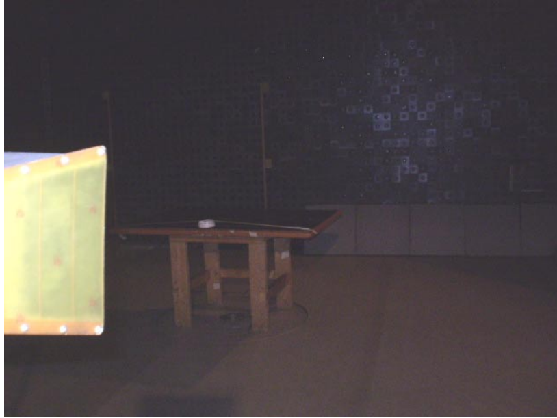
Photograph No.7 Setup for radiated emission measurements in the anechoic chamber above 1000 MHz range
