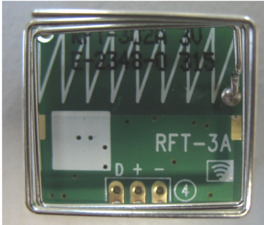
Photograph No.6 Detector RF module front view
