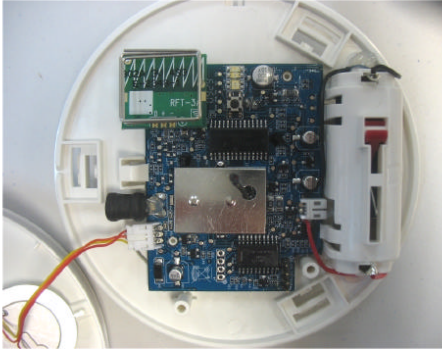
Photograph No.2 MCT-427 detector internal view
