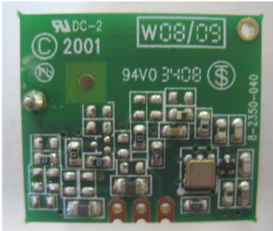
Photograph No.7 RF module PCB second side view
