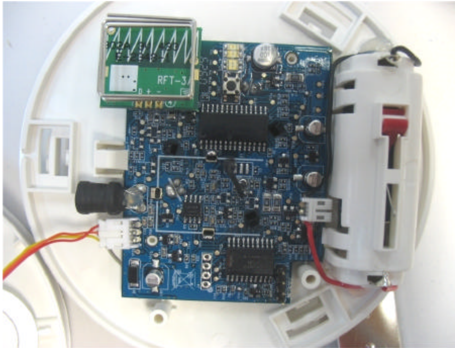
Photograph No.4 MCT-427 detector internal view with shield removed
