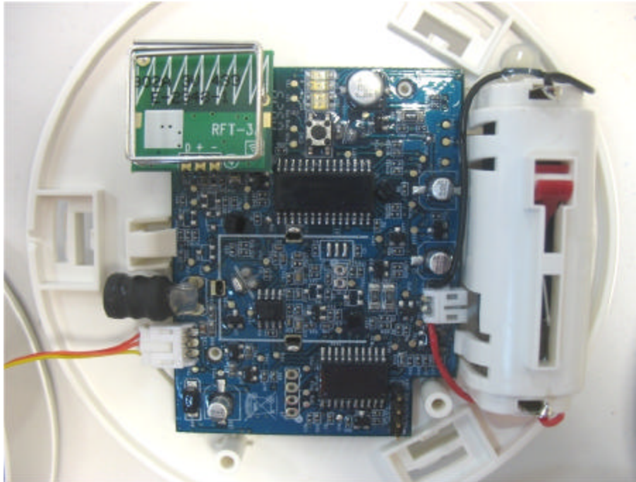
Photograph No.3 MCT-426 detector internal view with shield removed
