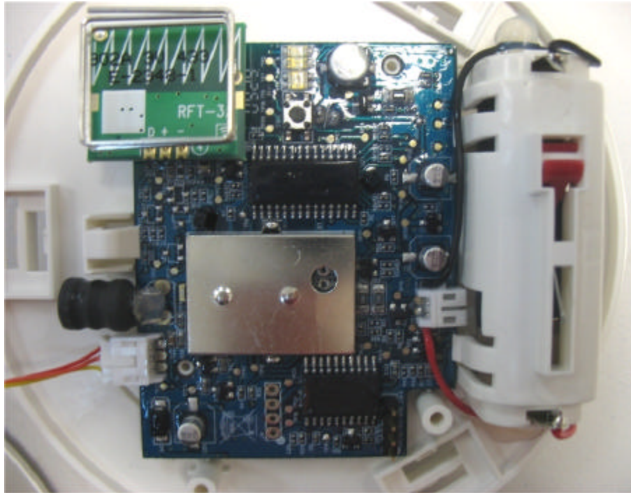
Photograph No.1 MCT-426 detector internal view
