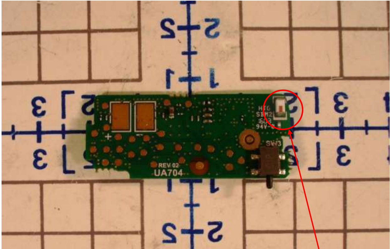
Illustration 4: EUT internal view – rear
