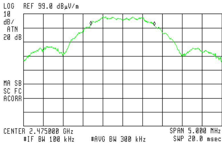
Figure 8. 2475MHz
