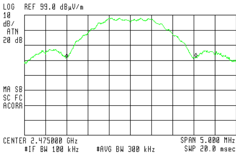
Figure 13. 2475MHz
