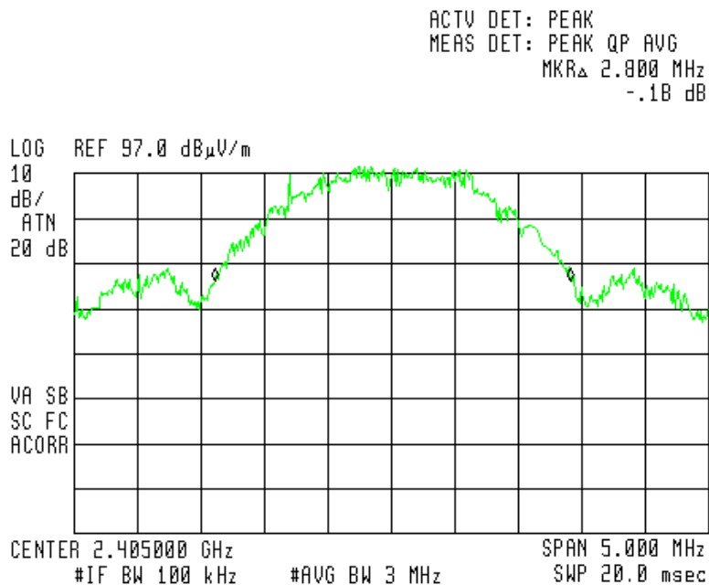
Figure 11. 2405MHz
