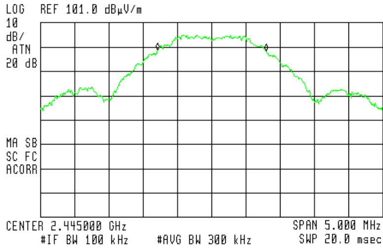
Figure 7. 2445MHz
