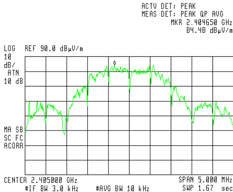
Figure 31 — 2405MHz
