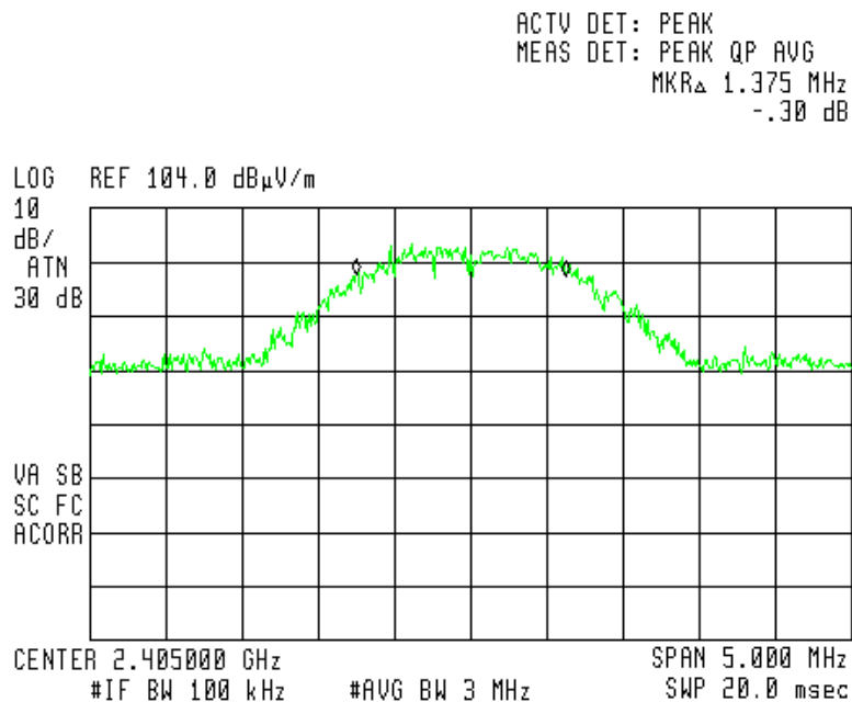
Figure 6. 2405MHz
