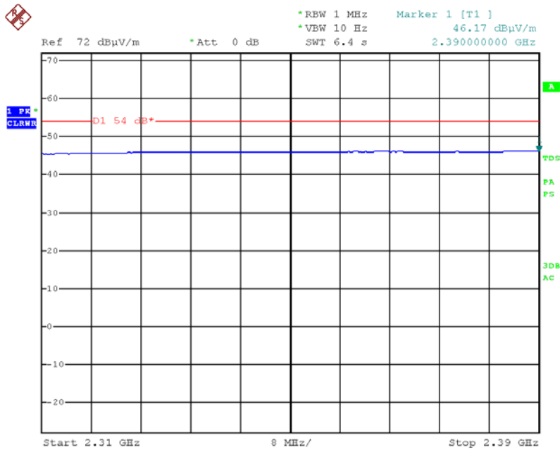
Figure 35. 2405 MHz ( Restricted Band Limit) Horizontal Peak
