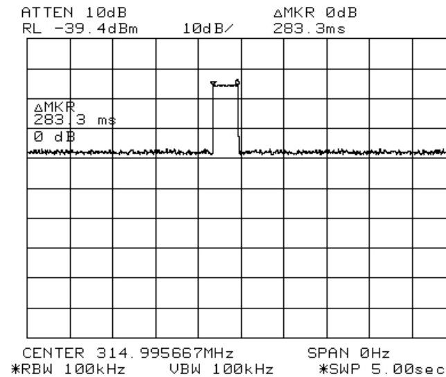
Figure 9. Automatic operated transmitter at low battery condition
