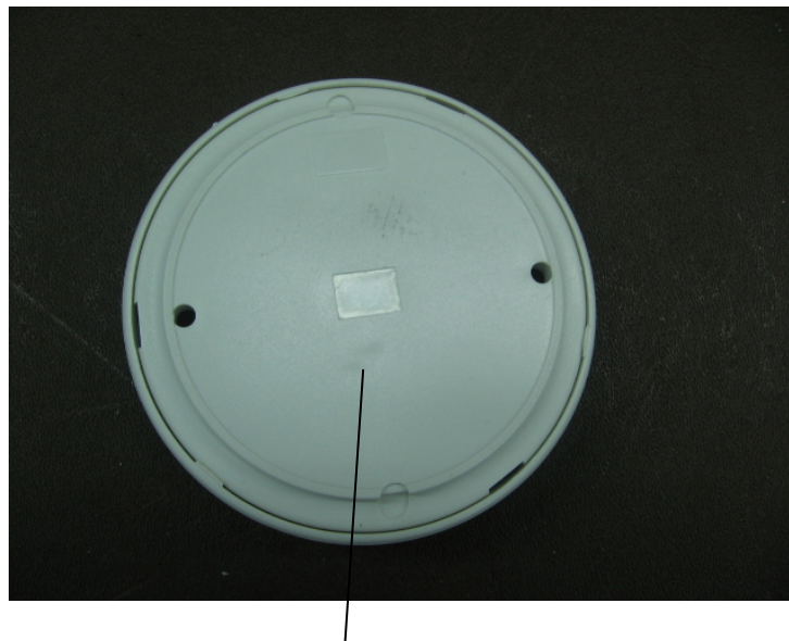
Figure 2. Location of Label on EUT
