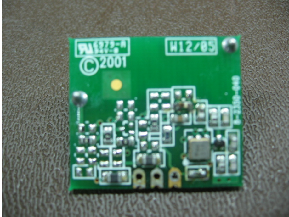
Figure 7: Bottom of RFT-3A
