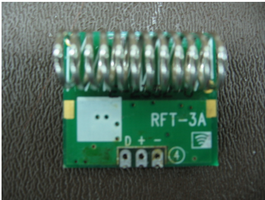
Figure 6: Top of RFT-3A
