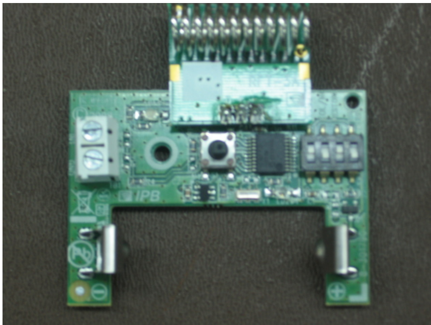
Figure 2: Top of PCB
