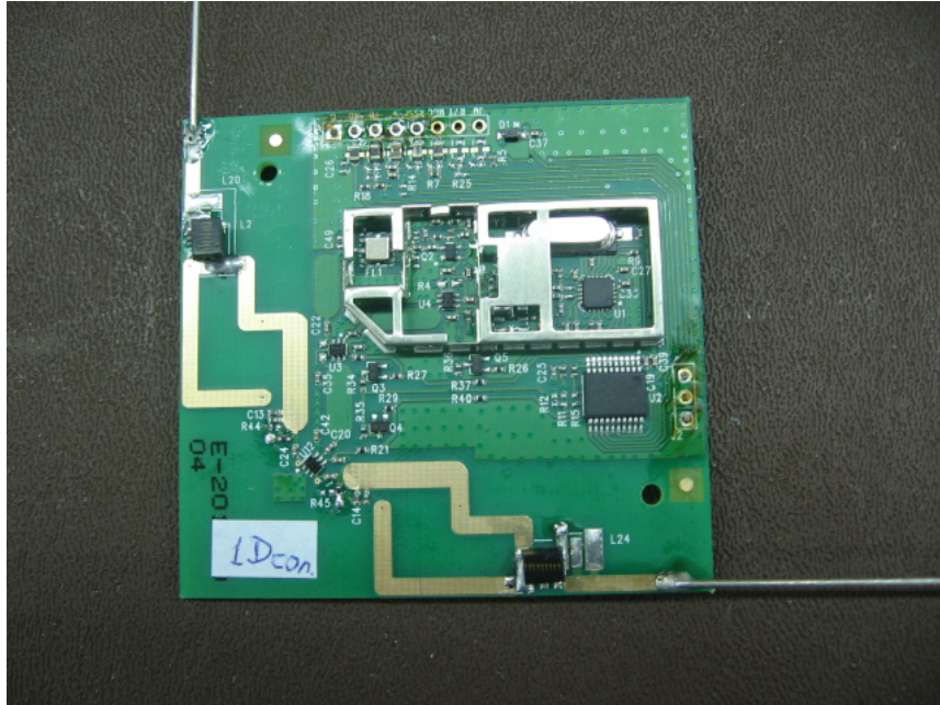
Figure 9: Top of Antenna PCB without cover
