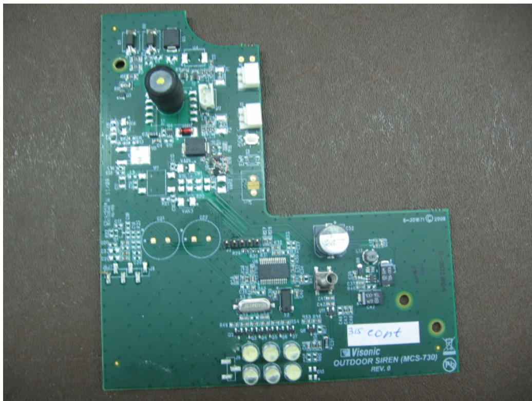
Figure 10: Top of main PCB
