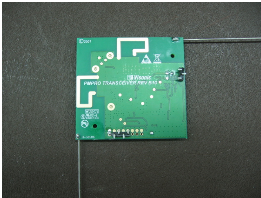
Figure 8: Bottom of Antenna PCB
