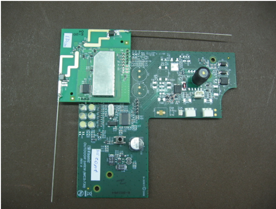
Figure 5: Top of PCB
