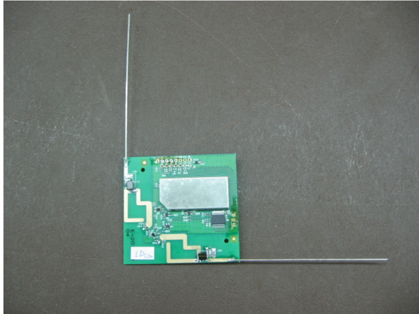
Figure 7: Top of Antenna PCB
