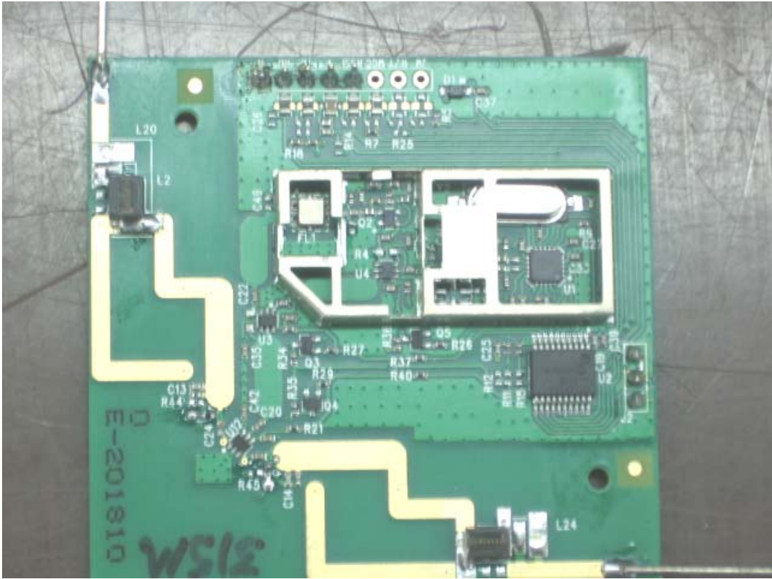
Figure 8: Top of Transceiver PCB
