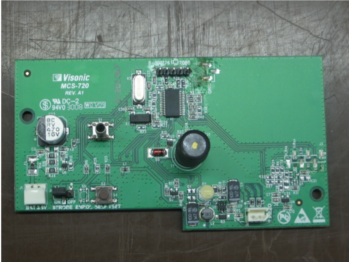
Figure 10: Top of PCB (Indoor Siren)
