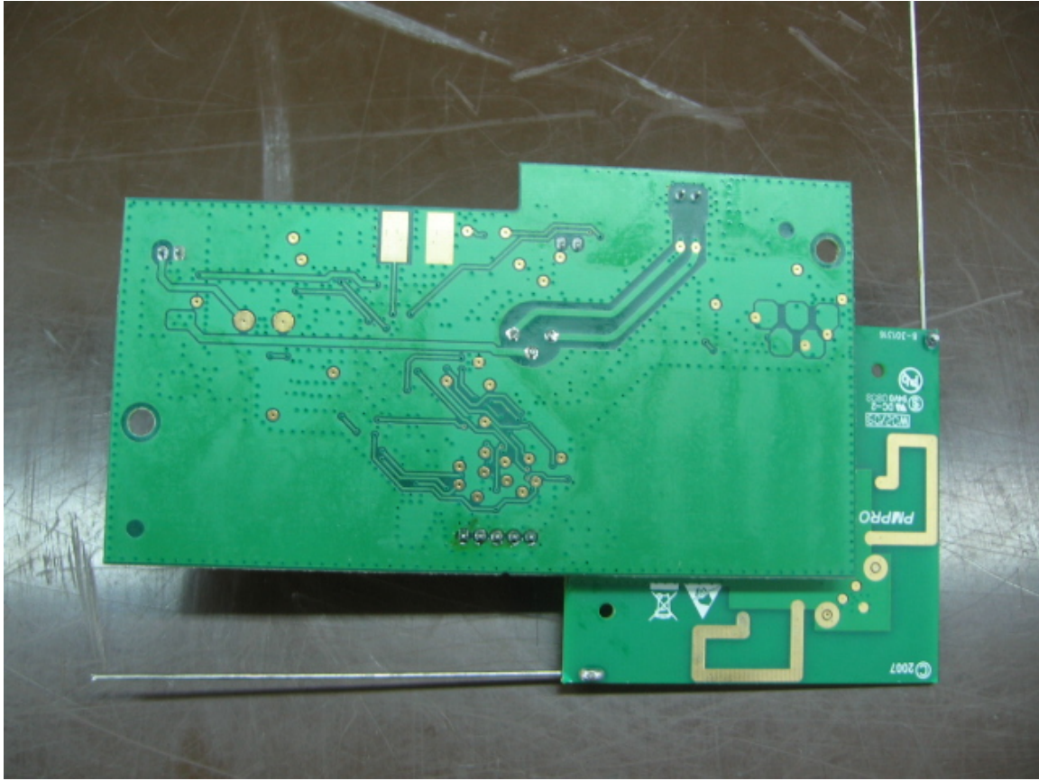
Figure 7: Bottom of PCB
