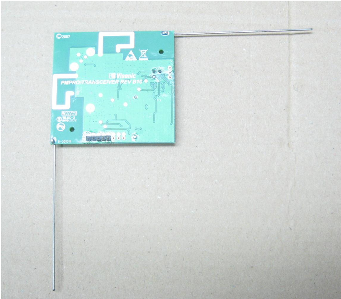
Figure 9: Bottom of Transceiver PCB
