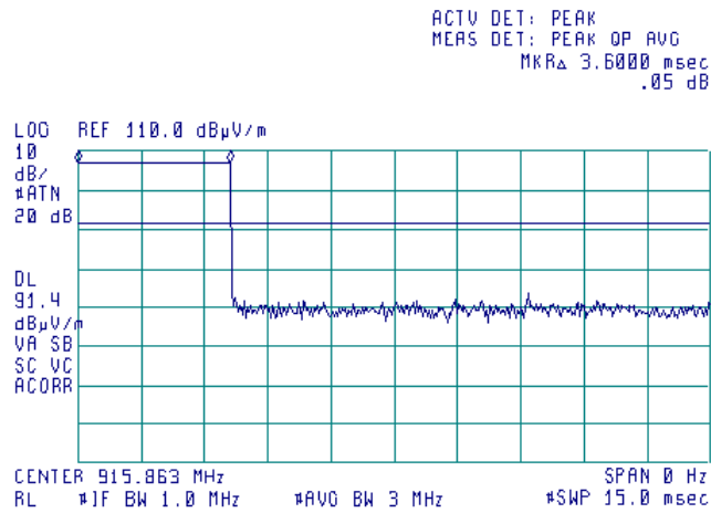
Plot 7.7.70 Transmission pulse period
