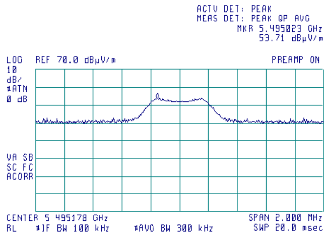
Plot 7.7.42 Radiated emission measurements at the sixth harmonic of mid carrier frequency
