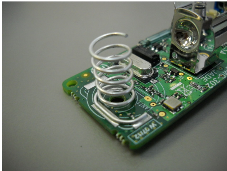
Photograph 7.8.1 Antenna assembly
