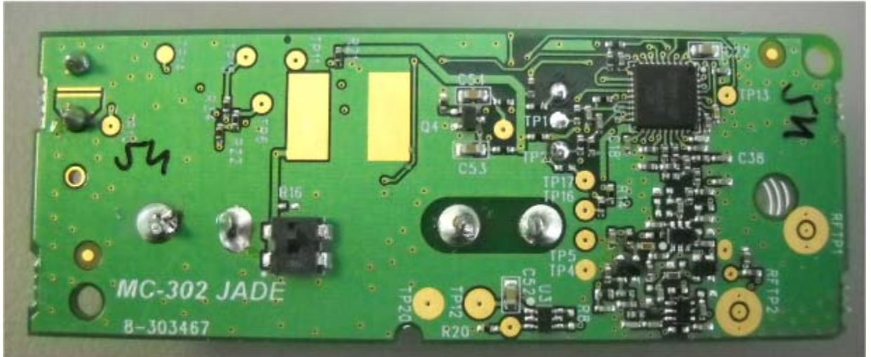
Photograph No.2 Magnetic contact device PCB rear side view
