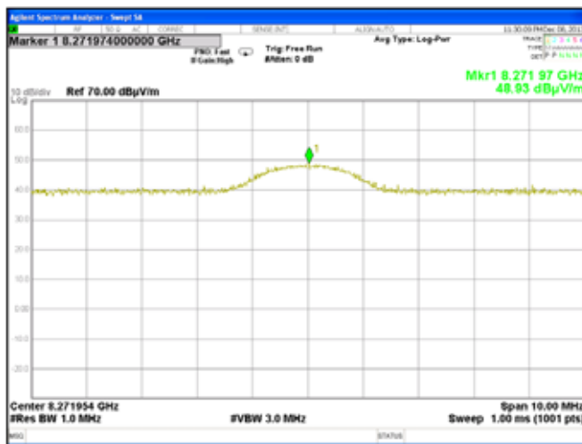
Plot 7.7.66 Radiated emission measurements at the ninth harmonic of high carrier frequency
