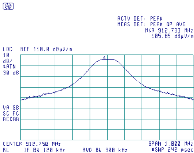
Plot 7.5.2 Field strength of carrier at low frequency, horizontal antenna polarization
