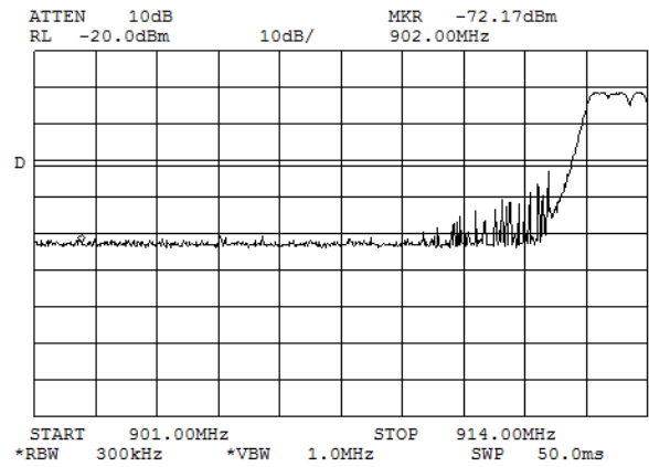
Plot 7.6.3 The highest band edge emission at low carrier frequency with hopping function enabled
