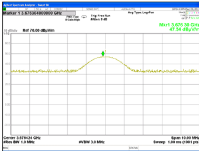
Plot 7.7.36 Radiated emission measurements at the fourth harmonic of high carrier frequency
