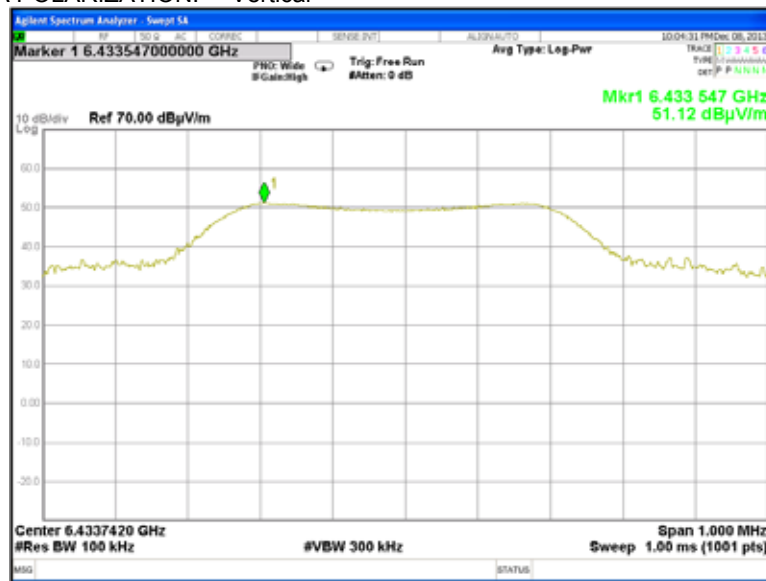
Plot 7.7.54 Radiated emission measurements at the seventh harmonic of high carrier frequency
