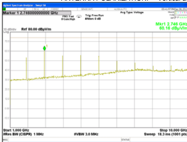
Plot 7.7.18 Radiated emission measurements from 1000 to 10000 MHz at the high carrier frequency
