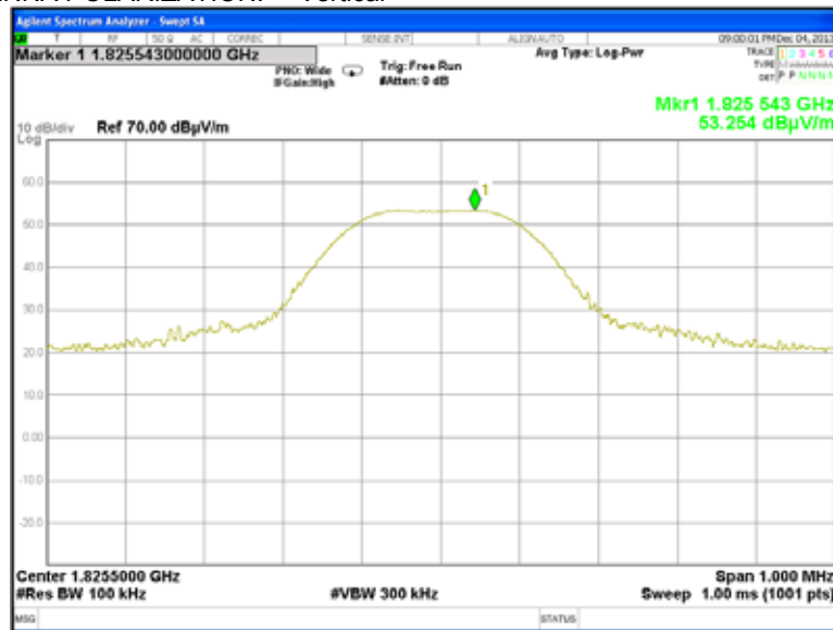
Plot 7.7.20 Radiated emission measurements at the second harmonic of low carrier frequency
