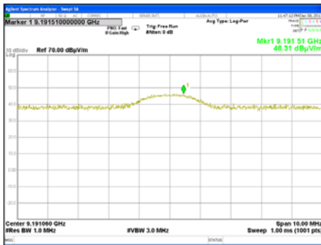
Plot 7.7.72 Radiated emission measurements at the tenth harmonic of high carrier frequency
