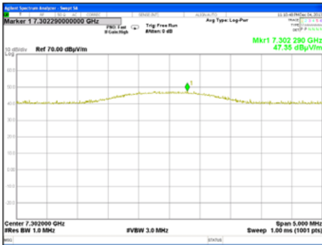
Plot 7.7.56 Radiated emission measurements at the eighth harmonic of low carrier frequency
