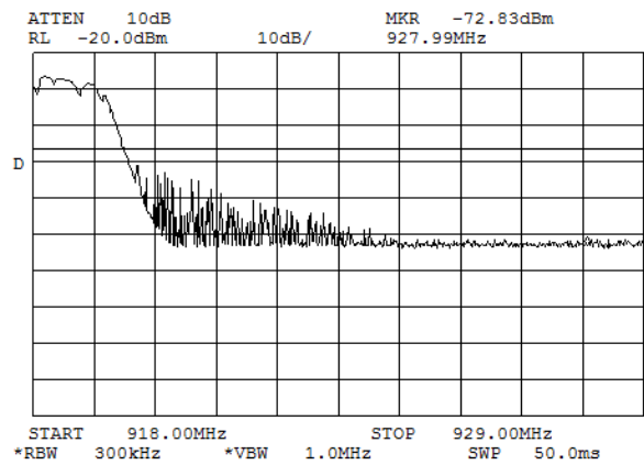
Plot 7.6.4 The highest band edge emission at high carrier frequency with hopping function enabled
