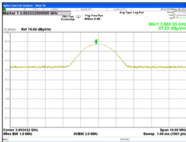
Plot 7.7.34 Radiated emission measurements at the fourth harmonic of mid carrier frequency
