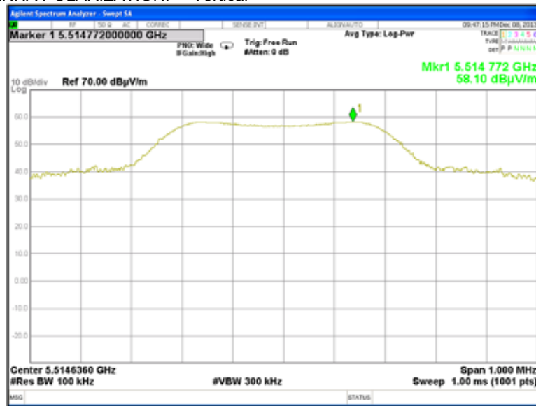
Plot 7.7.48 Radiated emission measurements at the sixth harmonic of high carrier frequency
