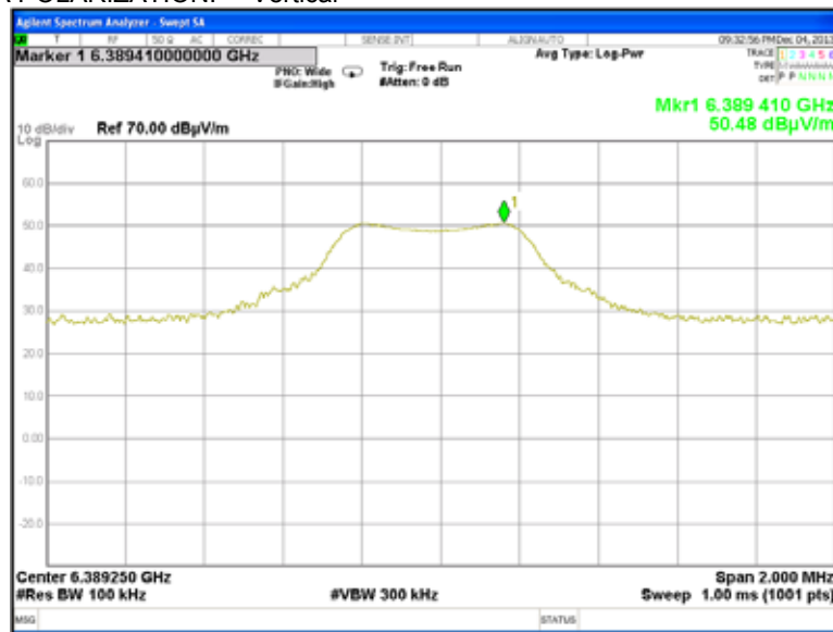
Plot 7.7.50 Radiated emission measurements at the seventh harmonic of low carrier frequency
