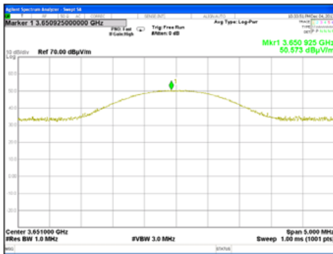
Plot 7.7.32 Radiated emission measurements at the fourth harmonic of low carrier frequency
