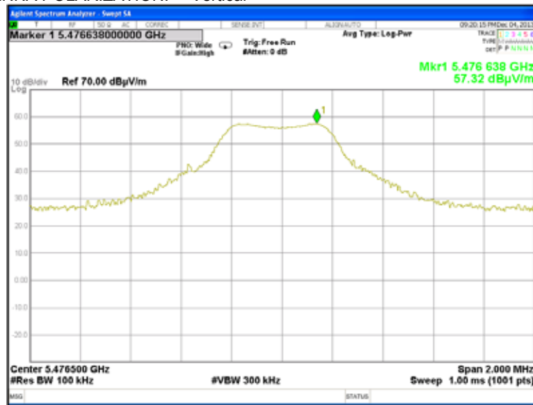
Plot 7.7.44 Radiated emission measurements at the sixth harmonic of low carrier frequency
