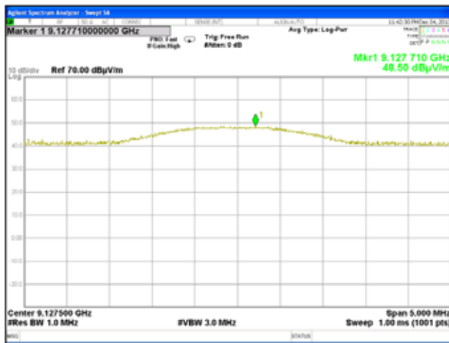
Plot 7.7.68 Radiated emission measurements at the tenth harmonic of low carrier frequency
