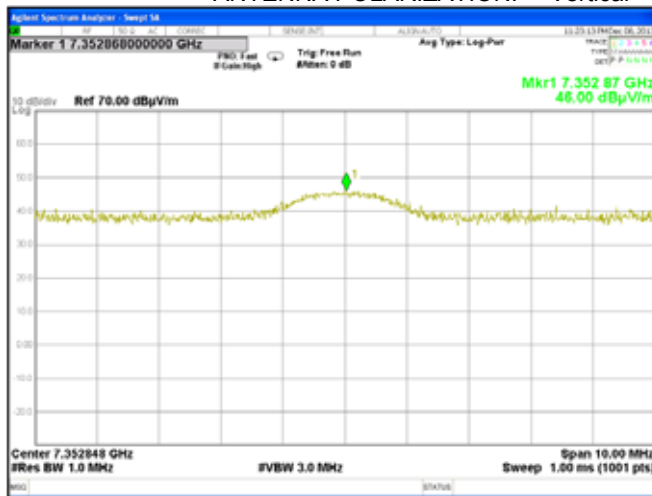
Plot 7.7.60 Radiated emission measurements at the eighth harmonic of high carrier frequency
