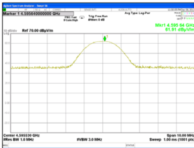
Plot 7.7.42 Radiated emission measurements at the fifth harmonic of high carrier frequency
