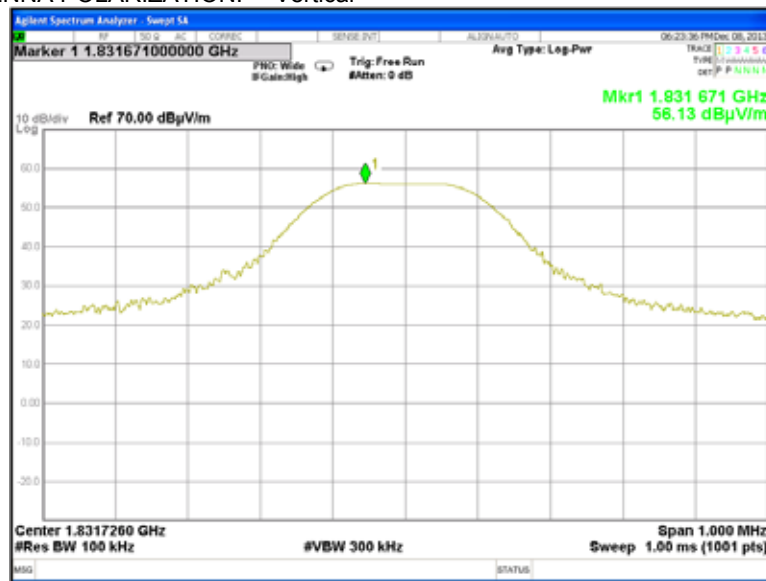
Plot 7.7.22 Radiated emission measurements at the second harmonic of mid carrier frequency
