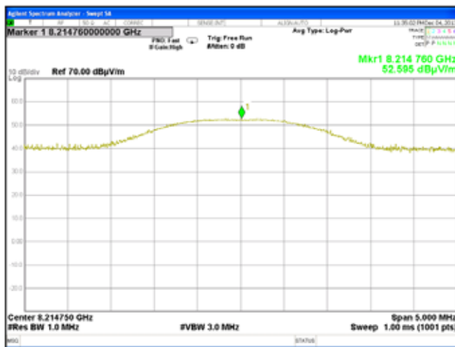
Plot 7.7.62 Radiated emission measurements at the ninth harmonic of low carrier frequency
