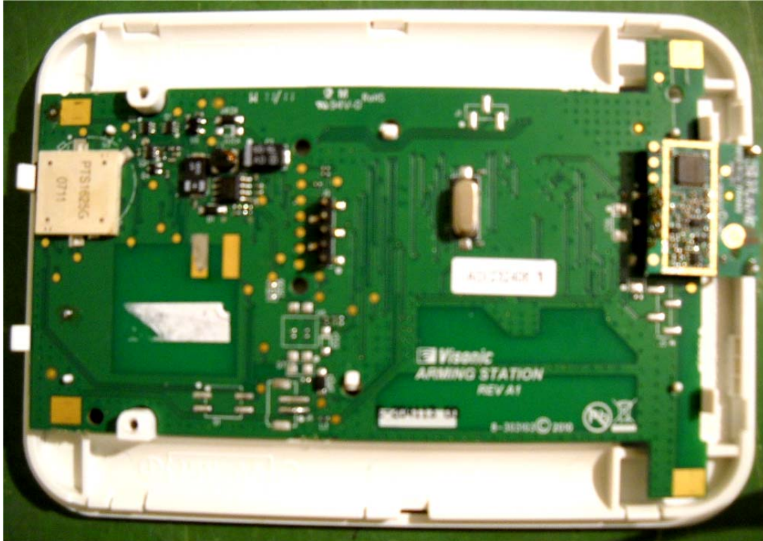
Photograph No.1 Touch screen keyprox internal view
