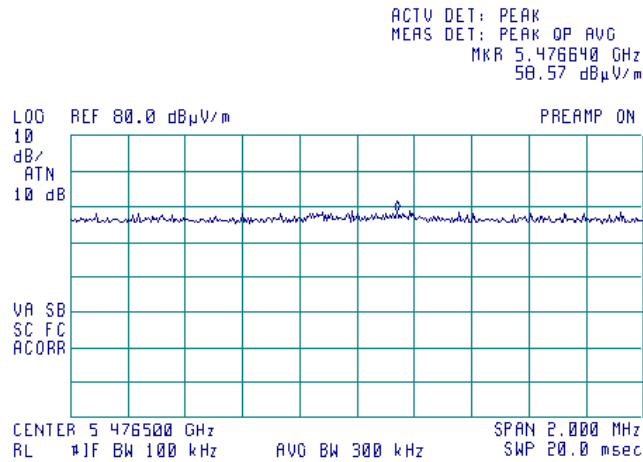
Plot 7.7.50 Radiated emission measurements at the sixth harmonic of low carrier frequency
