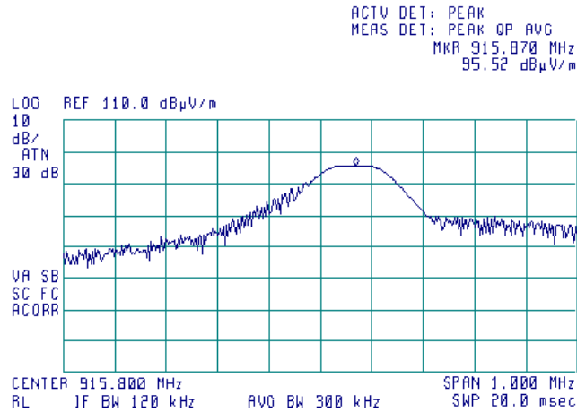
Plot 7.5.10 Field strength of carrier at mid frequency and EUT Y-axis position, horizontal antenna polarization
