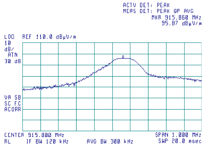
Plot 7.5.12 Field strength of carrier at mid frequency and EUT Z-axis position, horizontal antenna polarization
