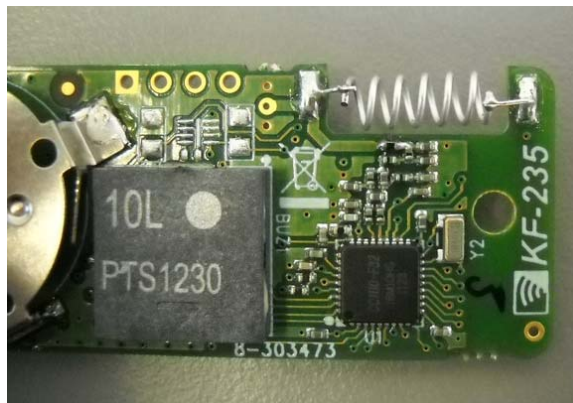
Photograph 7.8.1 Antenna assembly
