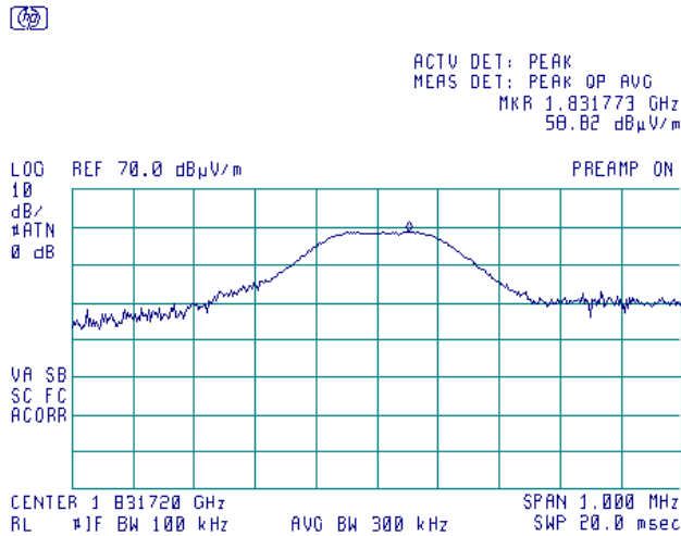
Plot 7.7.28 Radiated emission measurements at the second harmonic of mid carrier frequency
