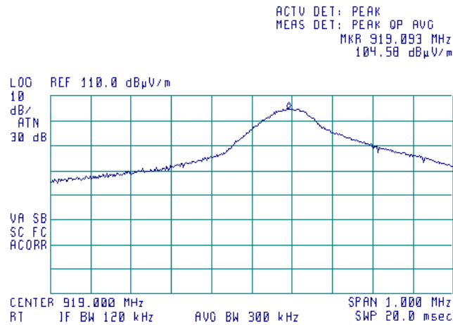
Plot 7.5.14 Field strength of carrier at high frequency and EUT X-axis position, horizontal antenna polarization
