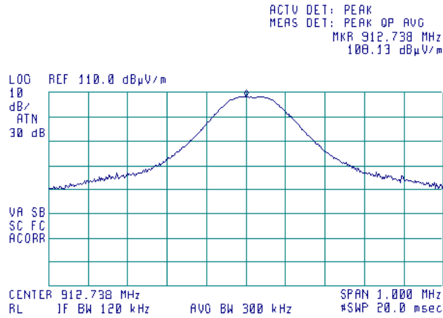
Plot 7.5.2 Field strength of carrier at low frequency and EUT X-axis position, horizontal antenna polarization
