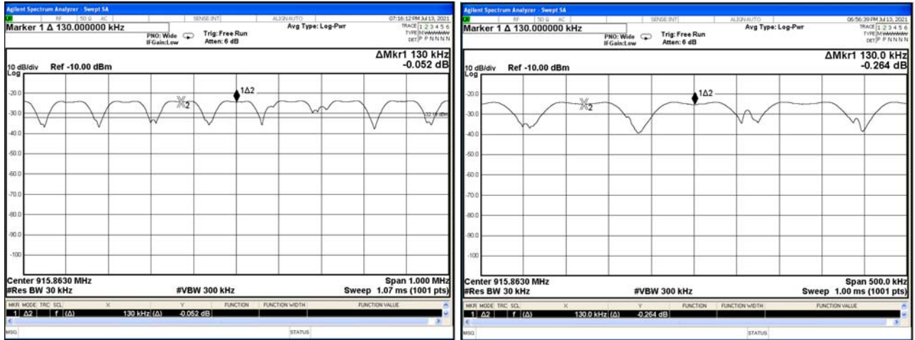
Plot 7.2.1 Carrier frequency separation
