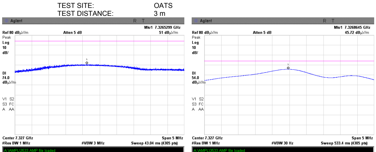
Plot 7.7.36 Radiated emission measurements at the eighth harmonic of mid carrier frequency
