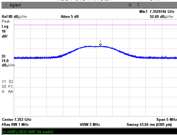
Plot 7.7.38 Radiated emission measurements at the tenth harmonic of low carrier frequency
