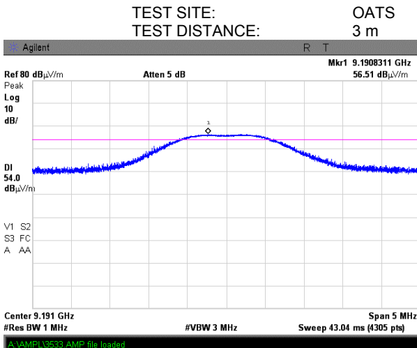
Plot 7.7.40 Radiated emission measurements at the tenth harmonic of high carrier frequency
