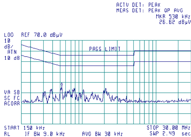
Plot 8.1.2 Conducted emissions at AC mains input port
