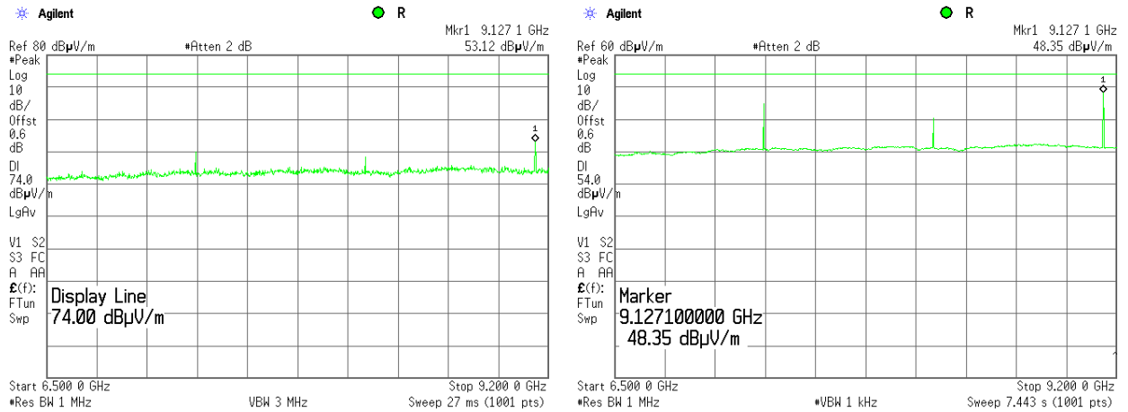
Plot 7.7.20 Radiated emission measurements from 6500 to 9200 MHz at the mid carrier frequency
