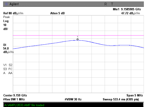
Plot 7.7.40 Radiated emission measurements at the tenth harmonic of high carrier frequency
