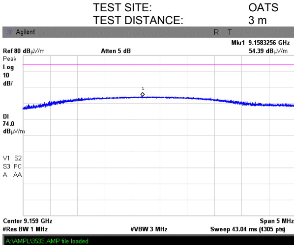
Plot 7.7.39 Radiated emission measurements at the tenth harmonic of mid carrier frequency
