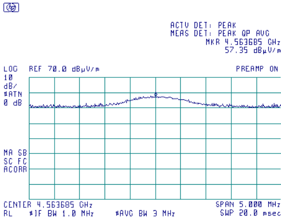
Plot 7.7.27 Radiated emission measurements at the fifth harmonic of mid carrier frequency
