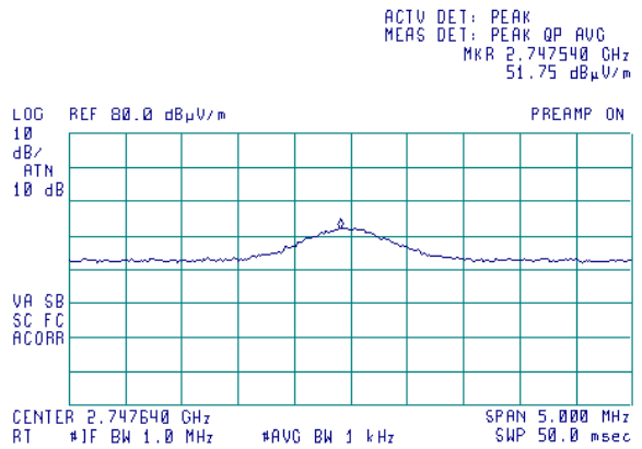
Plot 7.7.25 Radiated emission measurements at the third harmonic of high carrier frequency
