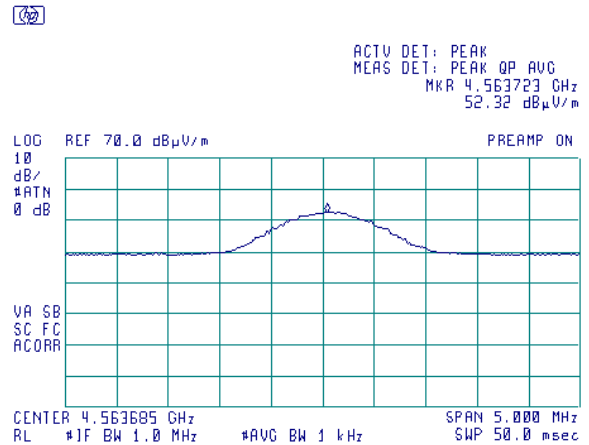
Plot 7.7.27 Radiated emission measurements at the fifth harmonic of mid carrier frequency
