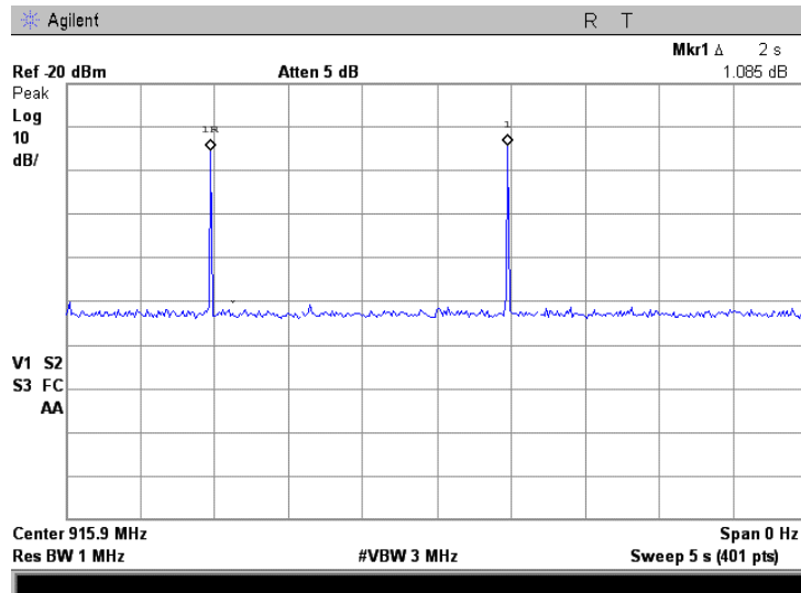
Plot 7.7.42 Transmission pulse period
