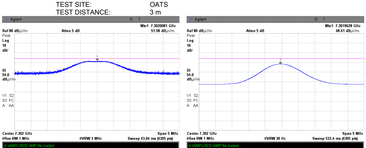
Plot 7.7.35 Radiated emission measurements at the eighth harmonic of low carrier frequency
