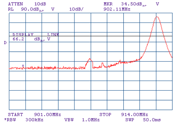
Plot 7.6.3 The highest band edge emission at low carrier frequency with hopping function disabled
