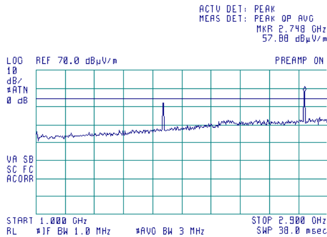
Plot 7.7.10 Radiated emission measurements from 1000 to 2900 MHz at the mid carrier frequency
