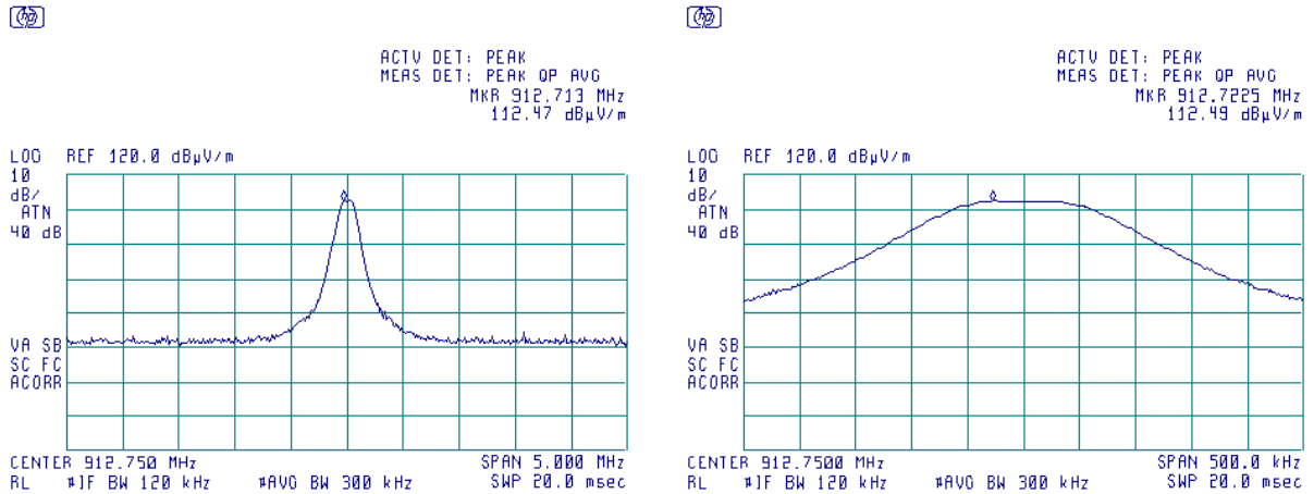
Plot 7.5.1 Field strength of carrier at low frequency in vertical antenna polarization
