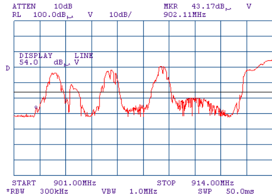
Plot 7.6.5 The highest band edge emission at low carrier frequency with hopping function enabled
