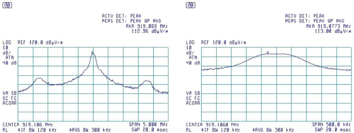
Plot 7.5.5 Field strength of carrier at high frequency in vertical antenna polarization
