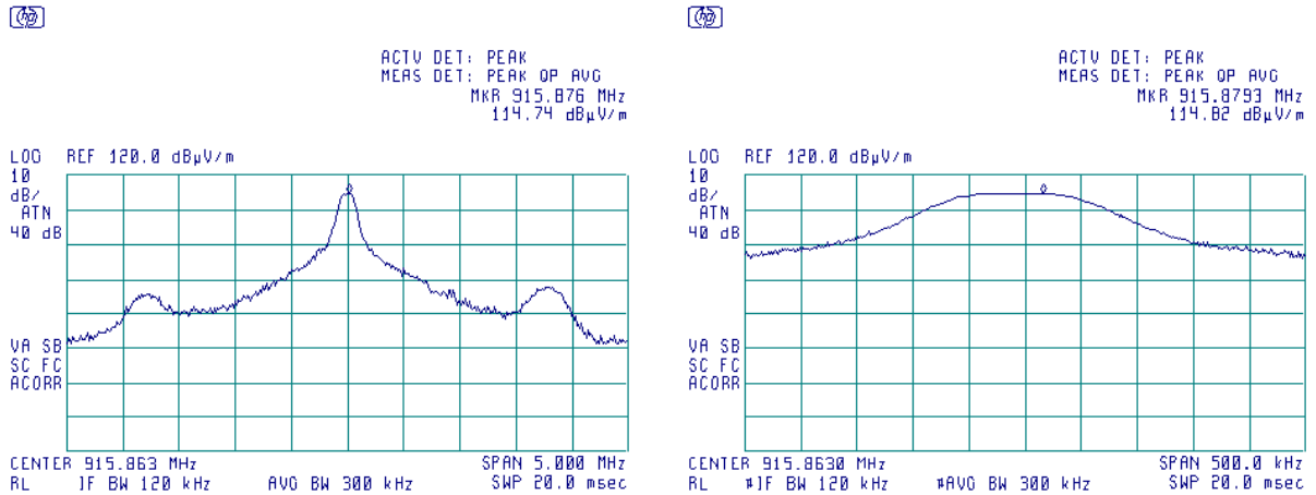
Plot 7.5.3 Field strength of carrier at mid frequency in vertical antenna polarization
