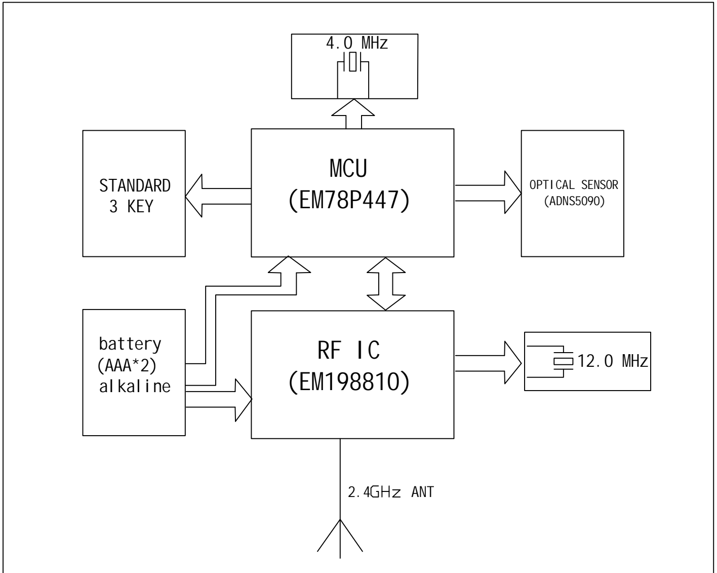
WIRELESS 2.4GHz MOUSE DIAGRAM:
