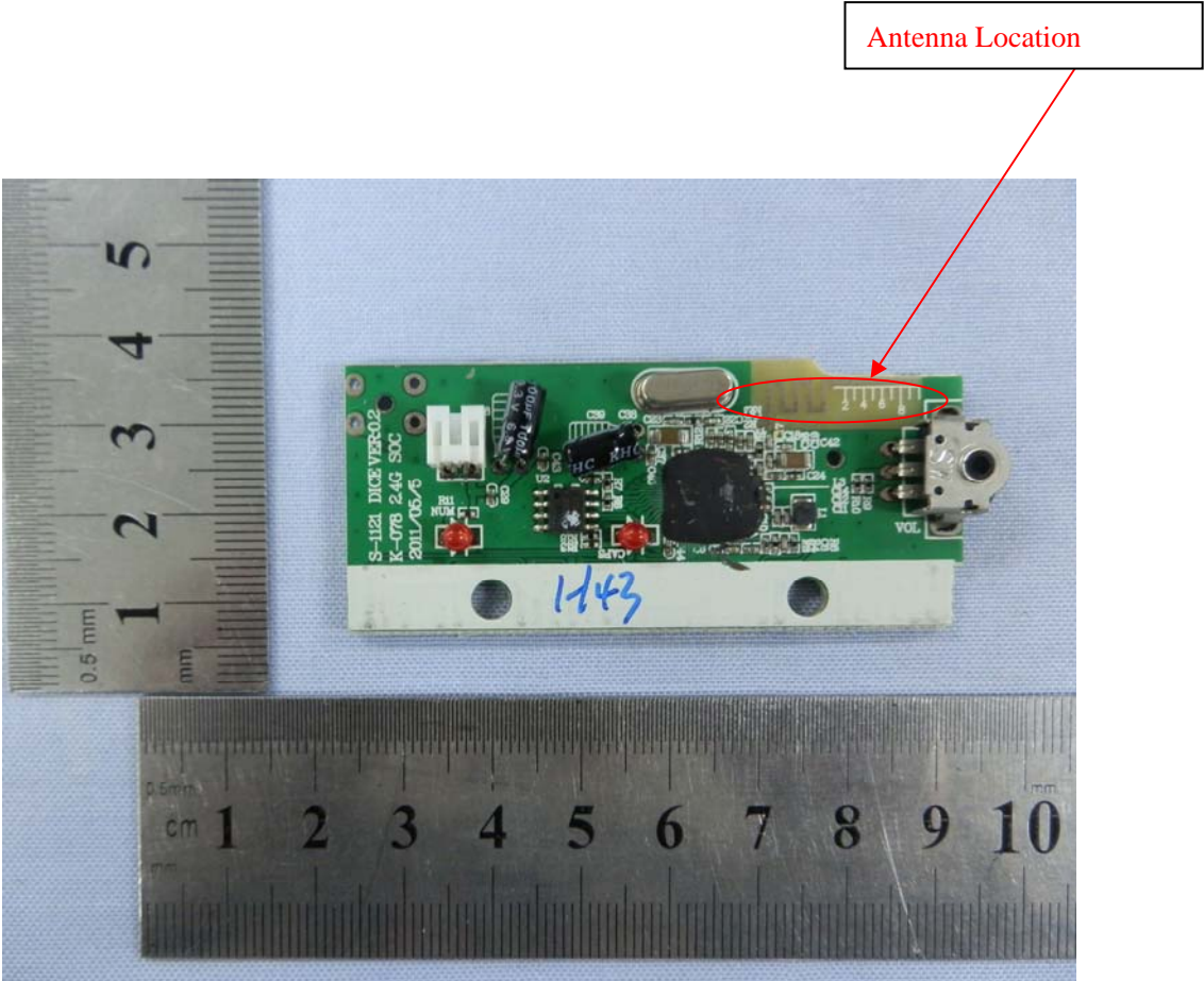
EUT - PCB View
