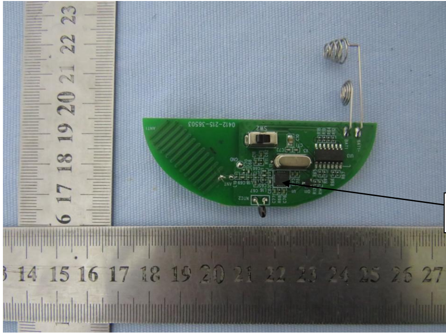
RF Chip
