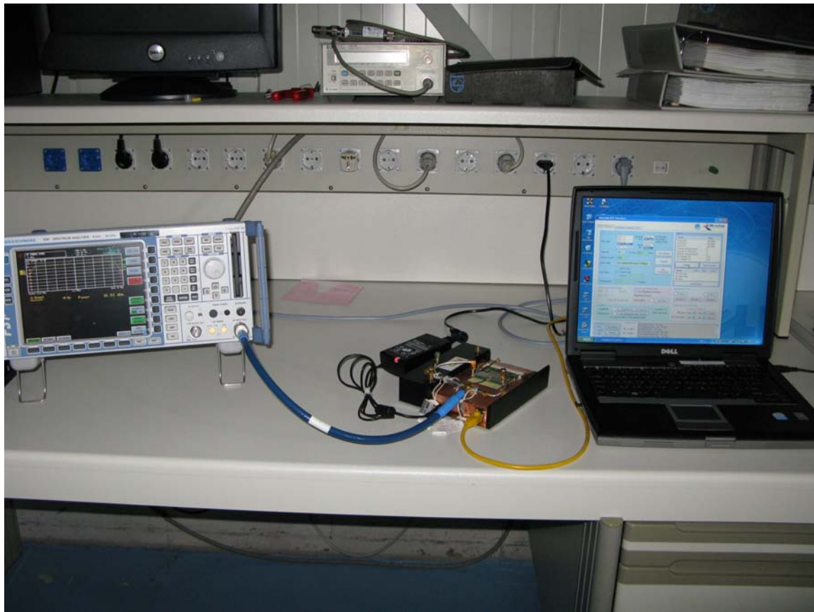
Photograph 4: Conducted RF measurement setup
