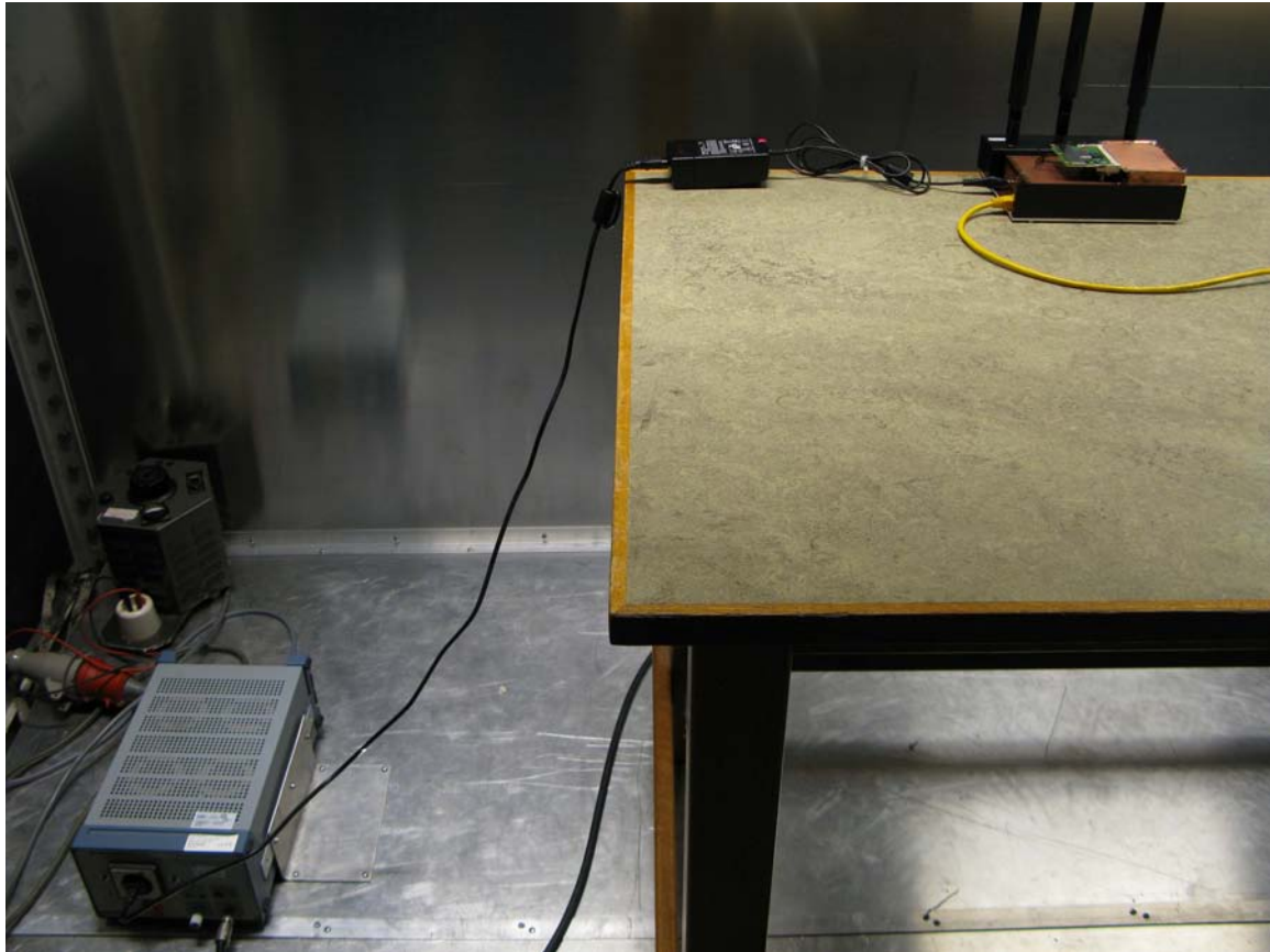
Photograph 1: Conducted emissions setup
