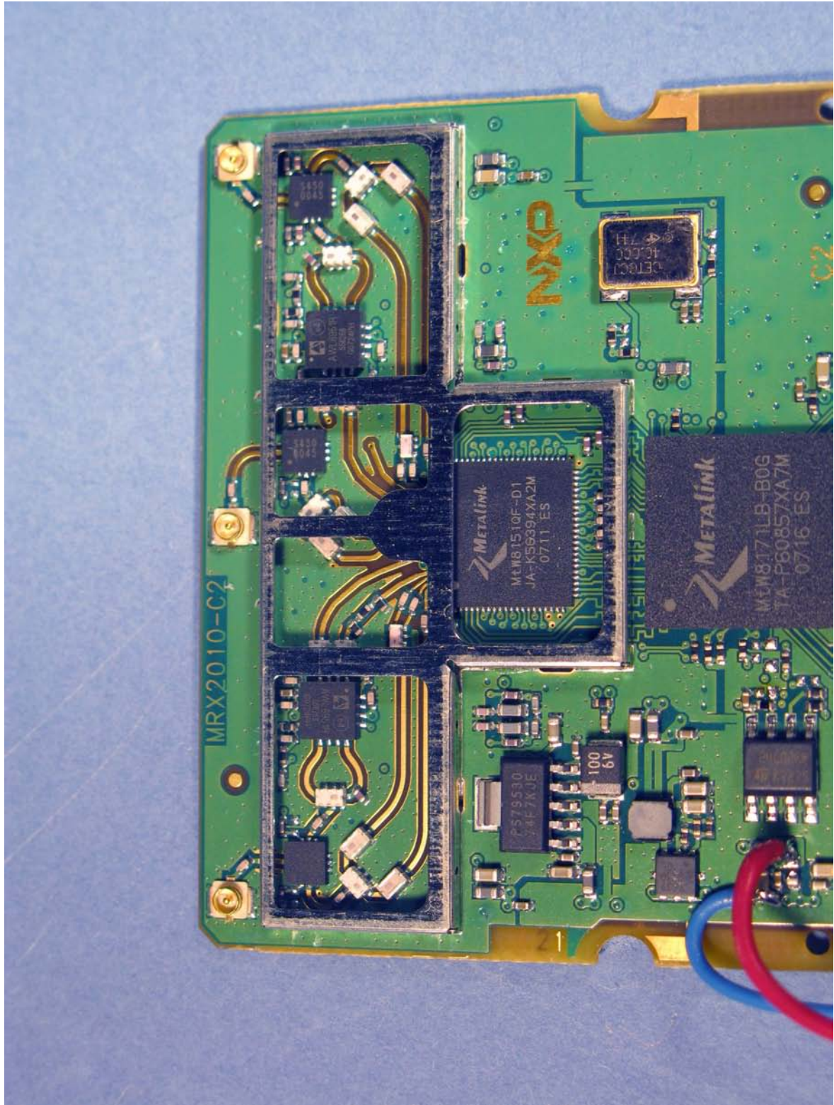
Photograph 1: MRX2010, inside metal shielding
