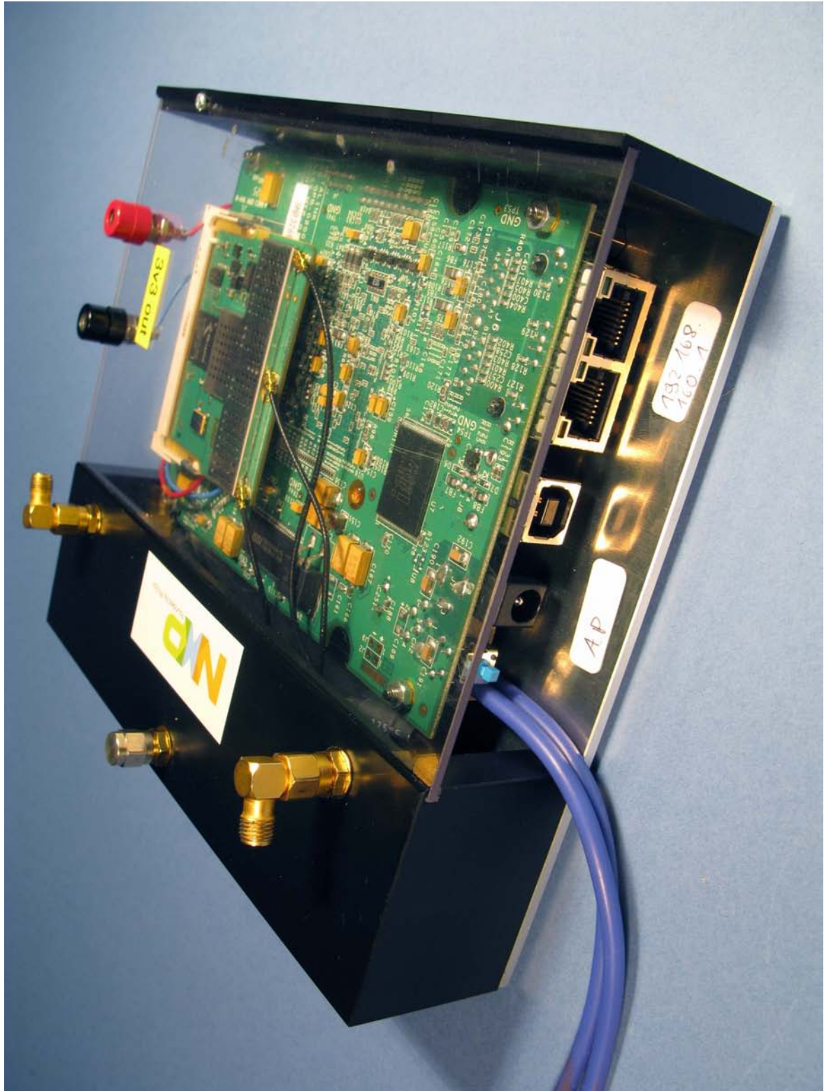
Photograph 2: Radio-measurements host, I/O
