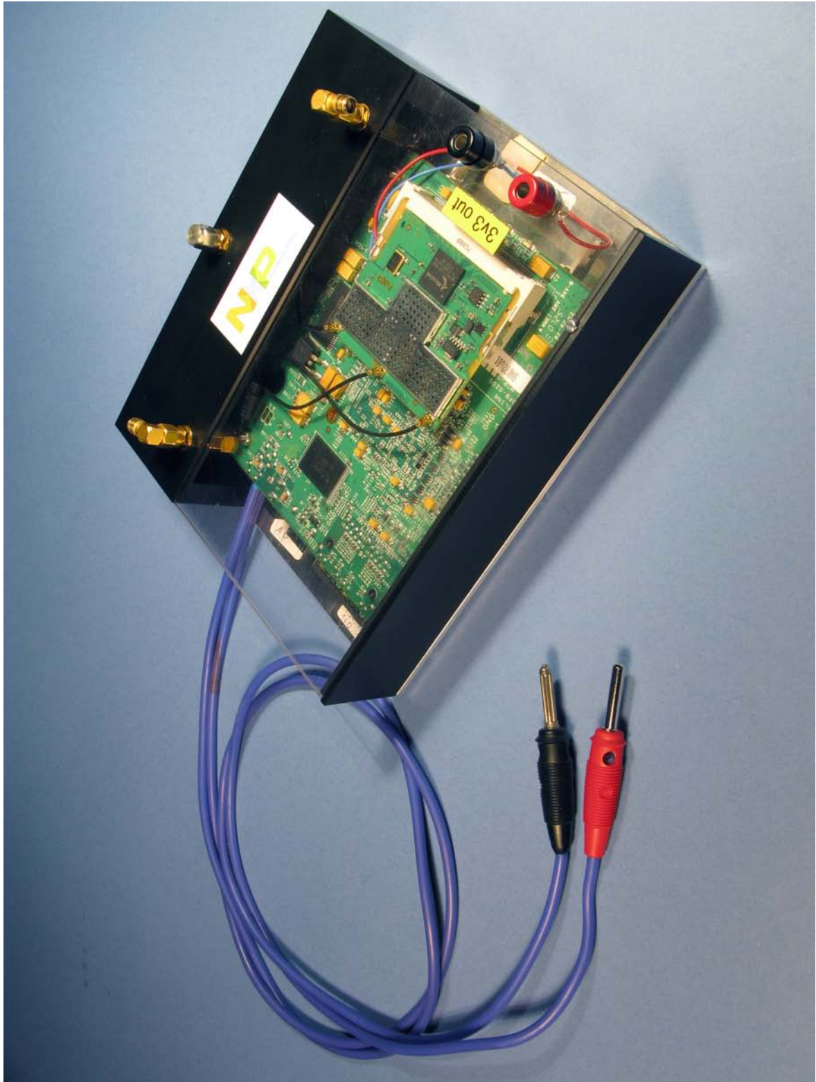
Photograph 1: MRX2010 inserted in radio-measurements host.
