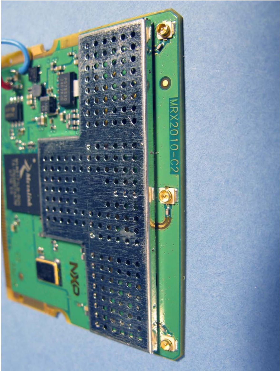
Photograph 7: MRX2010, antenna connectors
