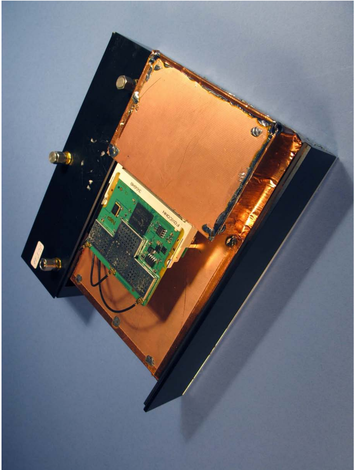
Photograph 3: MRX2010 inserted in radiated-measurements host
