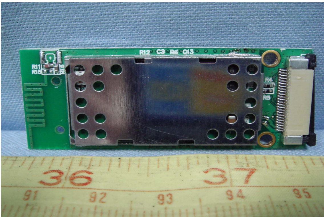
PCB Antenna
