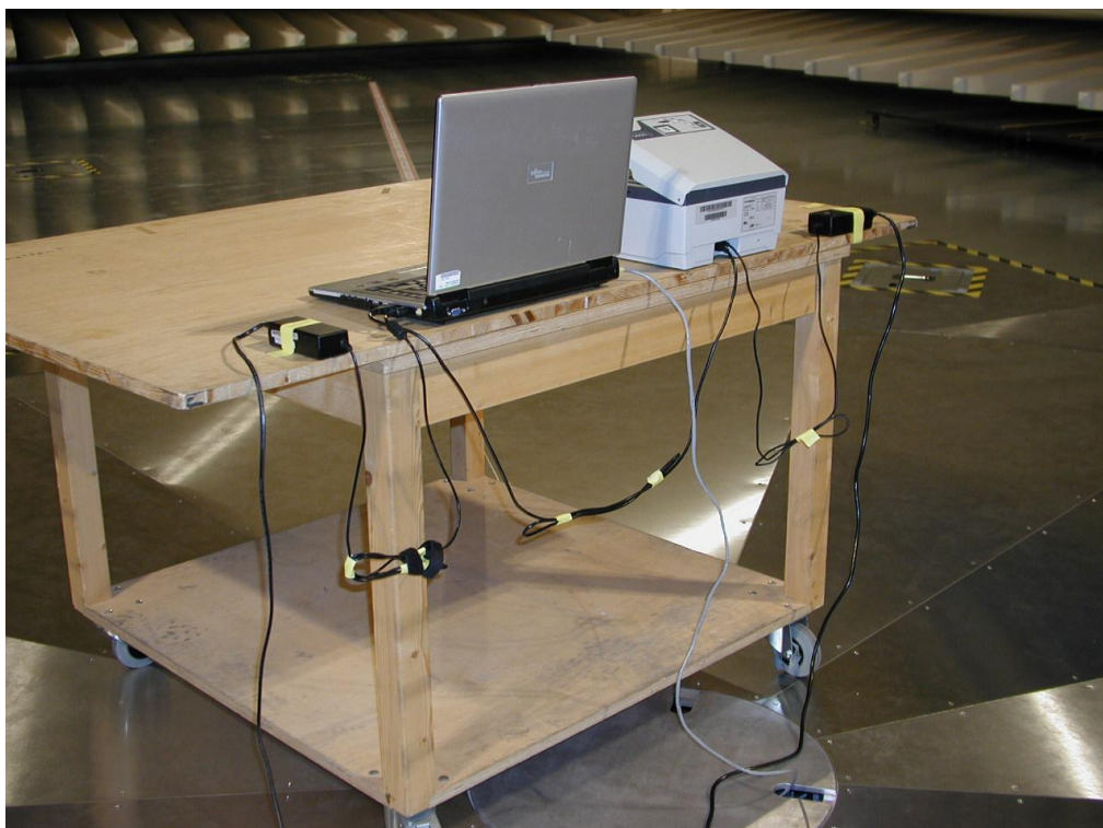
Figure 4 Arrangement for the measurement of radiated emissions
