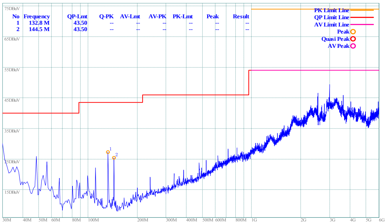
(Plot C: Test Antenna Horizontal)
