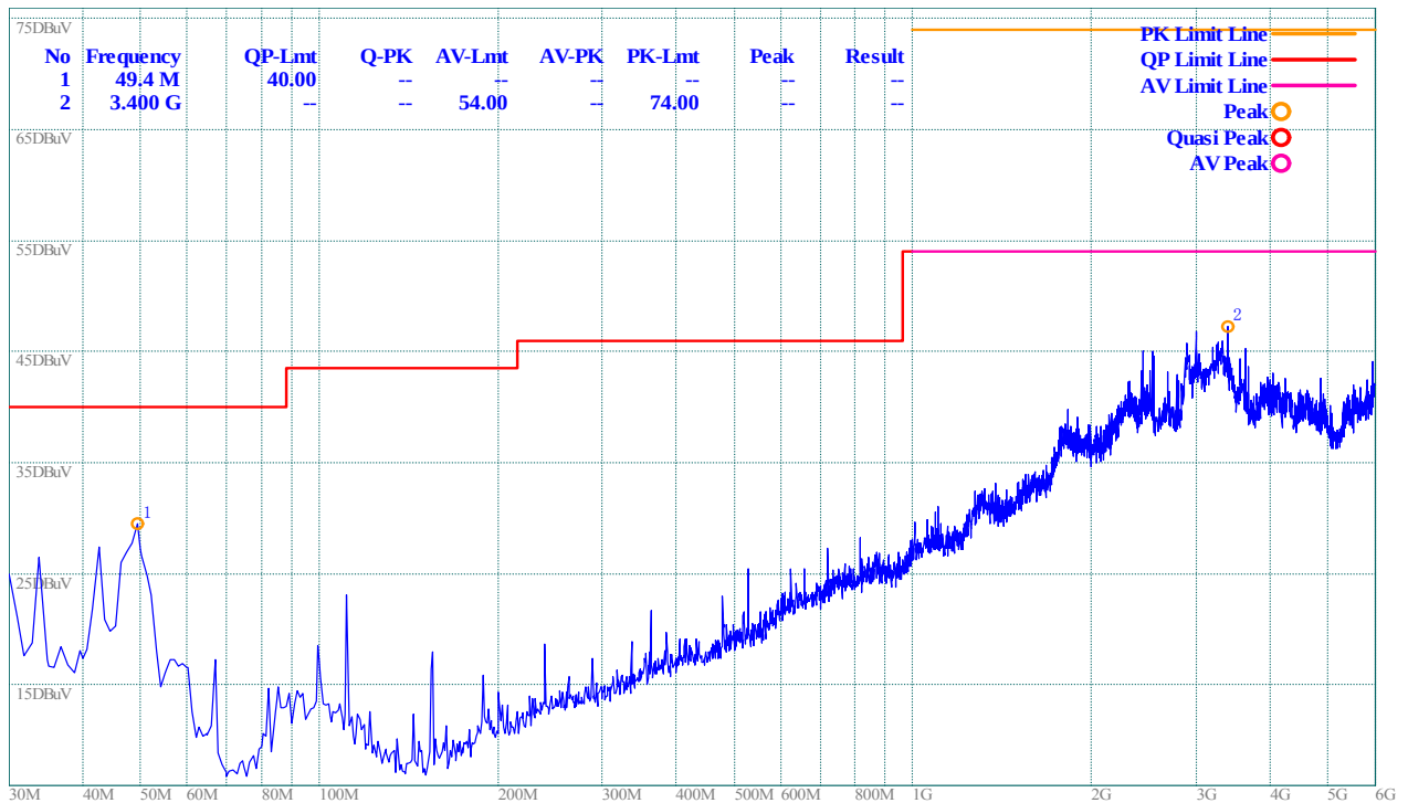
(Plot B: Test Antenna Vertical)
