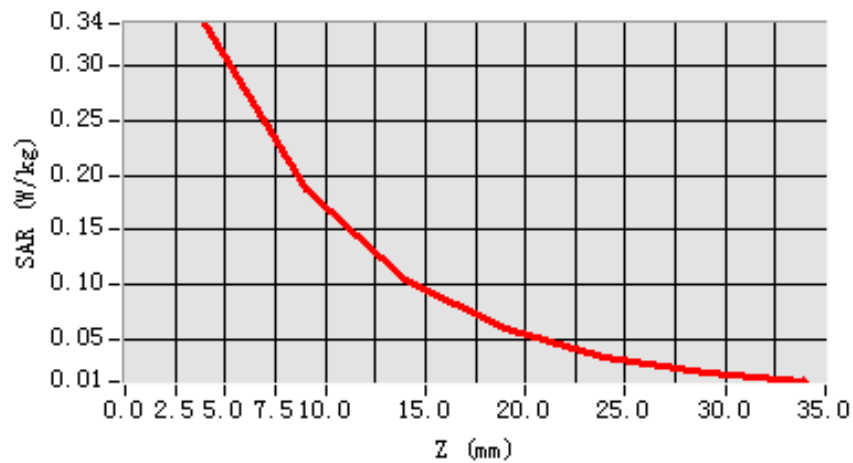
SAR, Z Axis Scan (X = -10, Y = -32)
