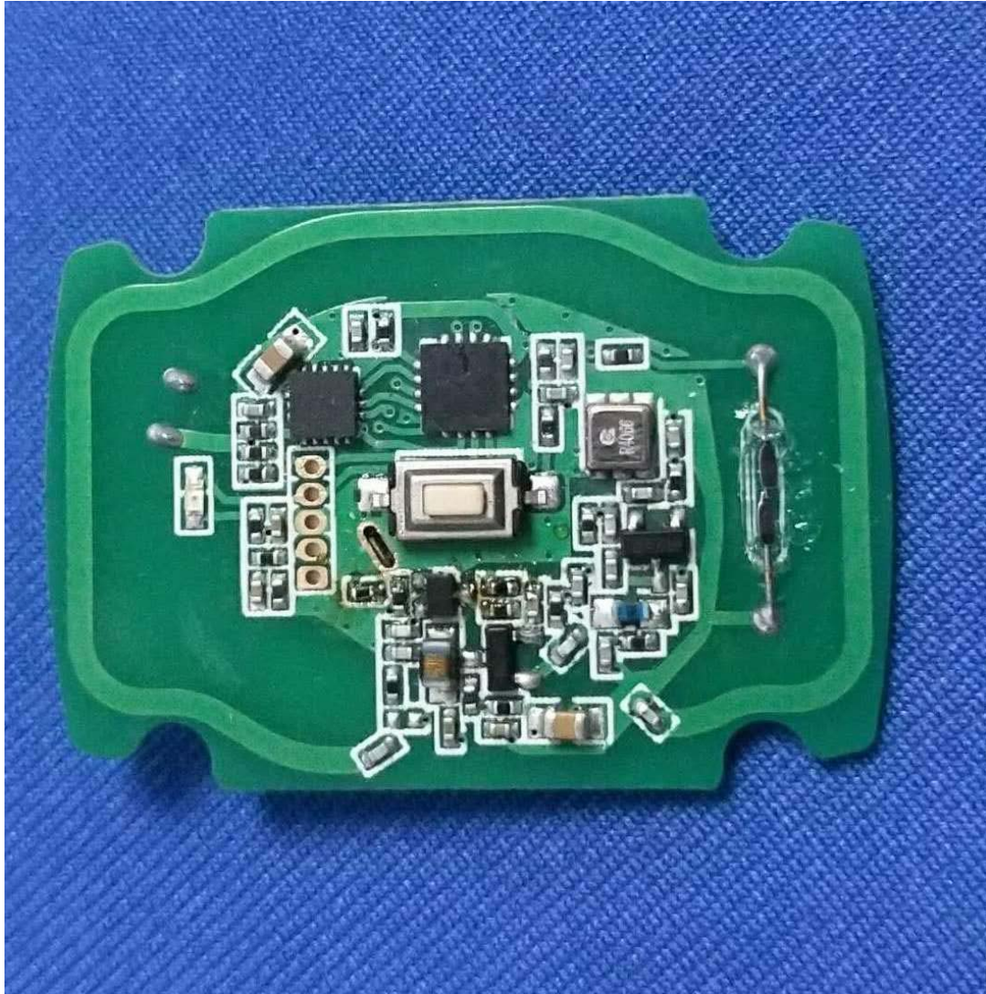
Figure 13 Inside of the EUT
